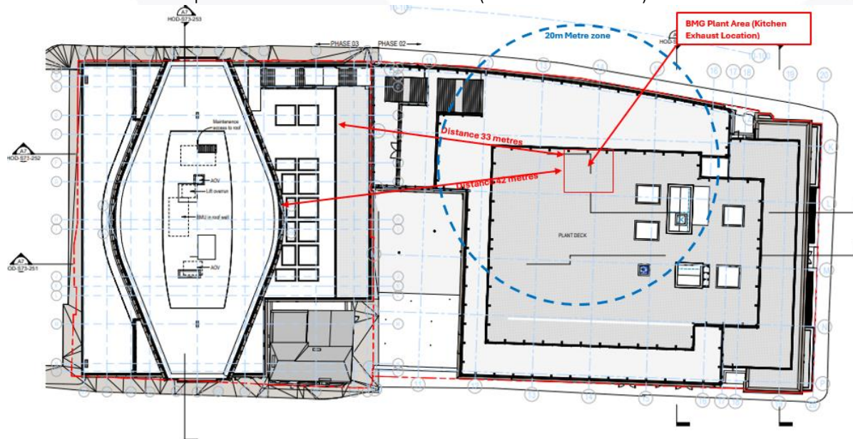
A7 SITE ROOF PLAN 1:200
