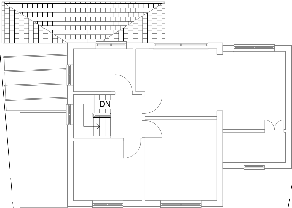
3 - First Floor 1 : 100
