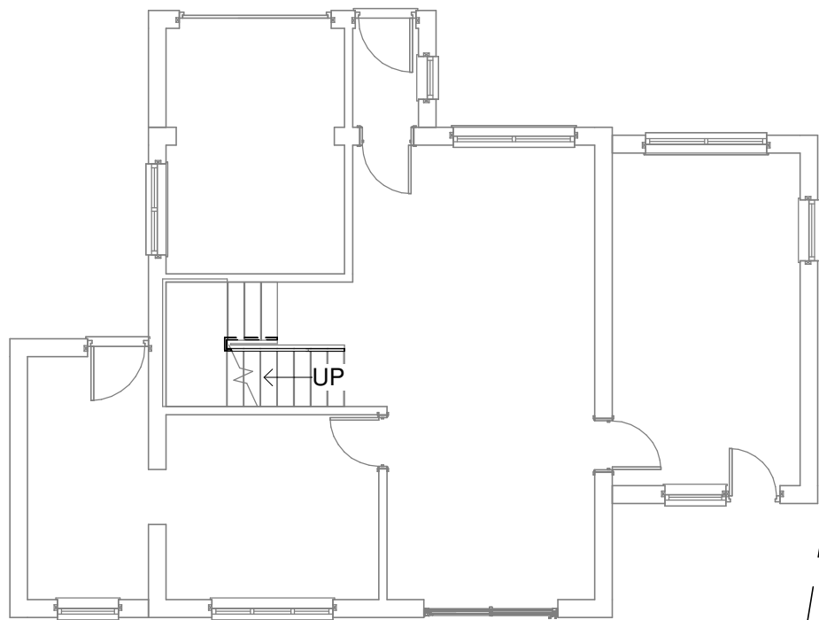
1 - Ground Floor 1 : 100
