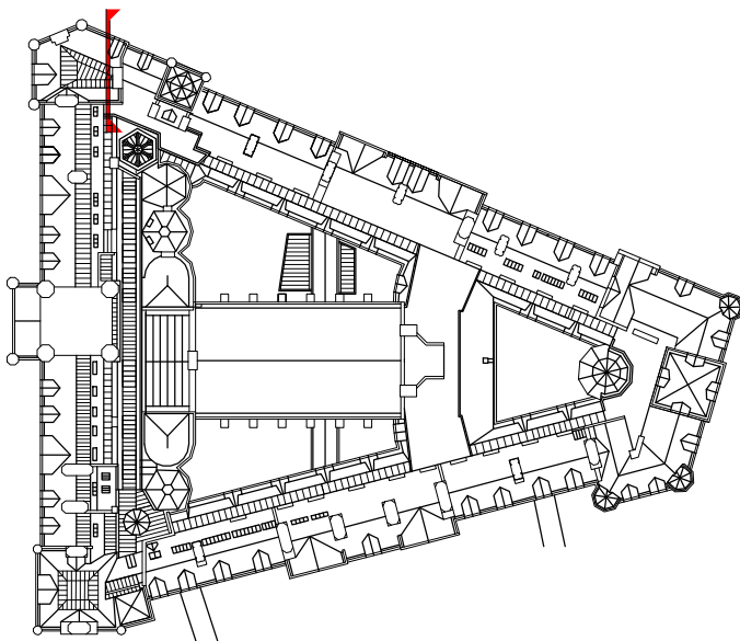
Key plan_Section BT 1 : 1250
