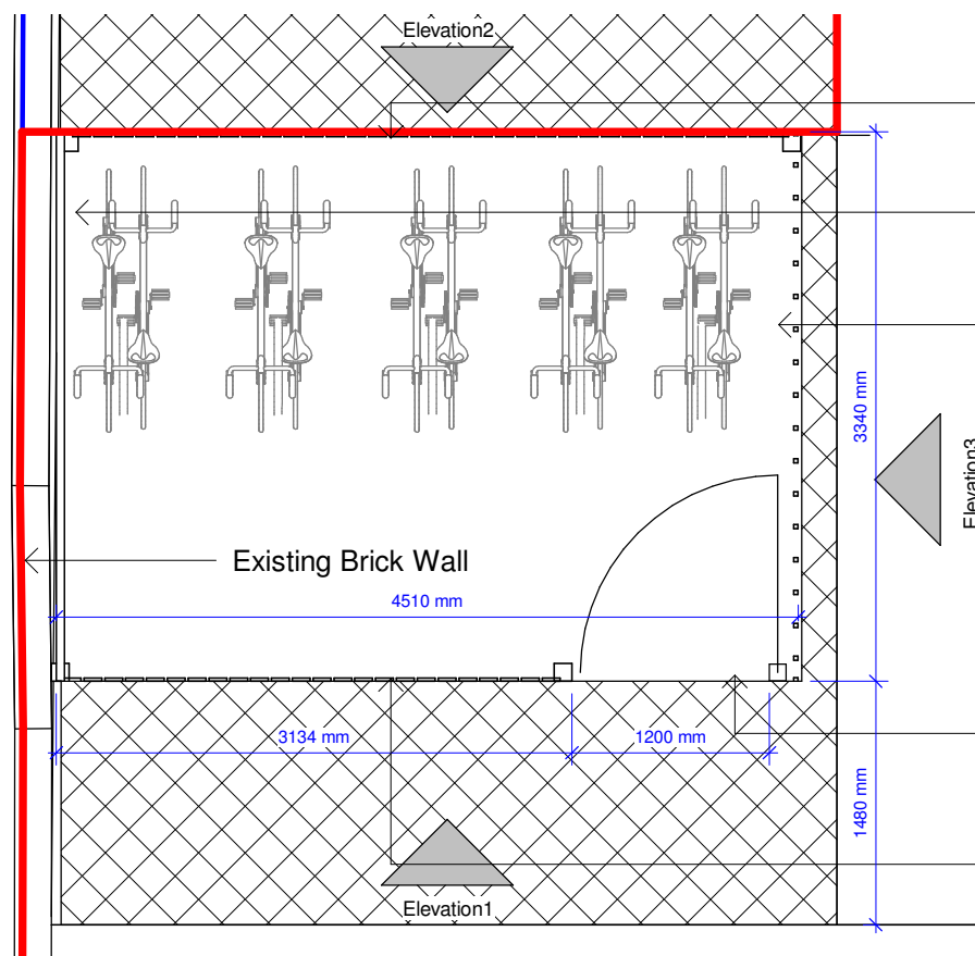
1 Bike Store - Plan 1 : 50
