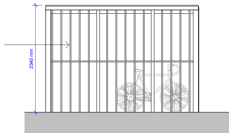
5 Bike Store - Elevation 3 1 : 50
