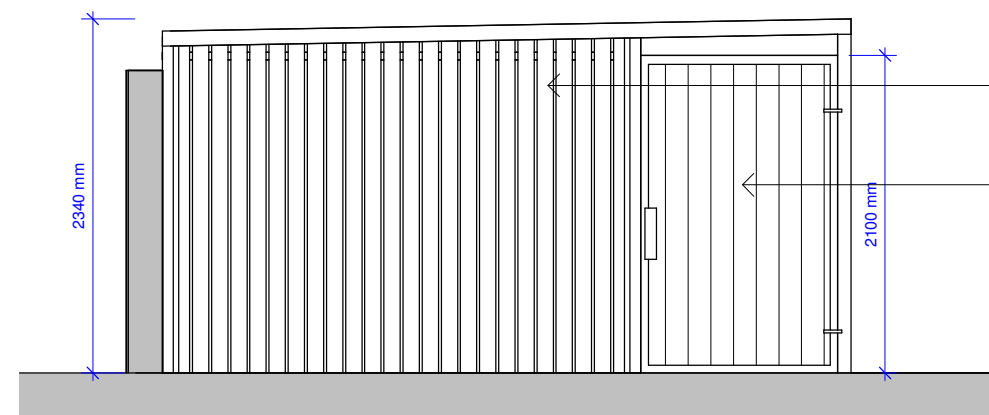
2 Bike Store - Elevation 1 1 : 50
