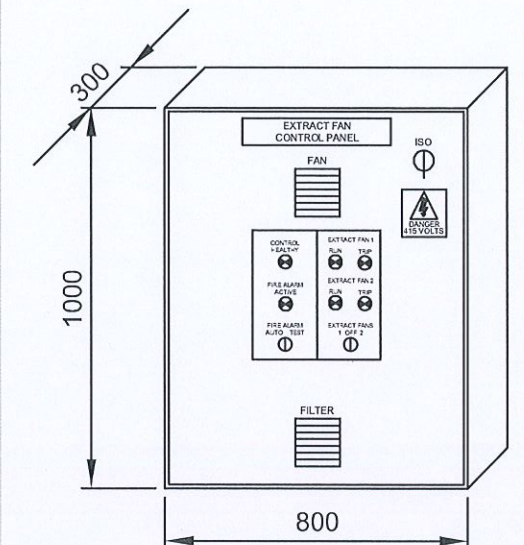
CONTROL PANEL DIMENSIONS
