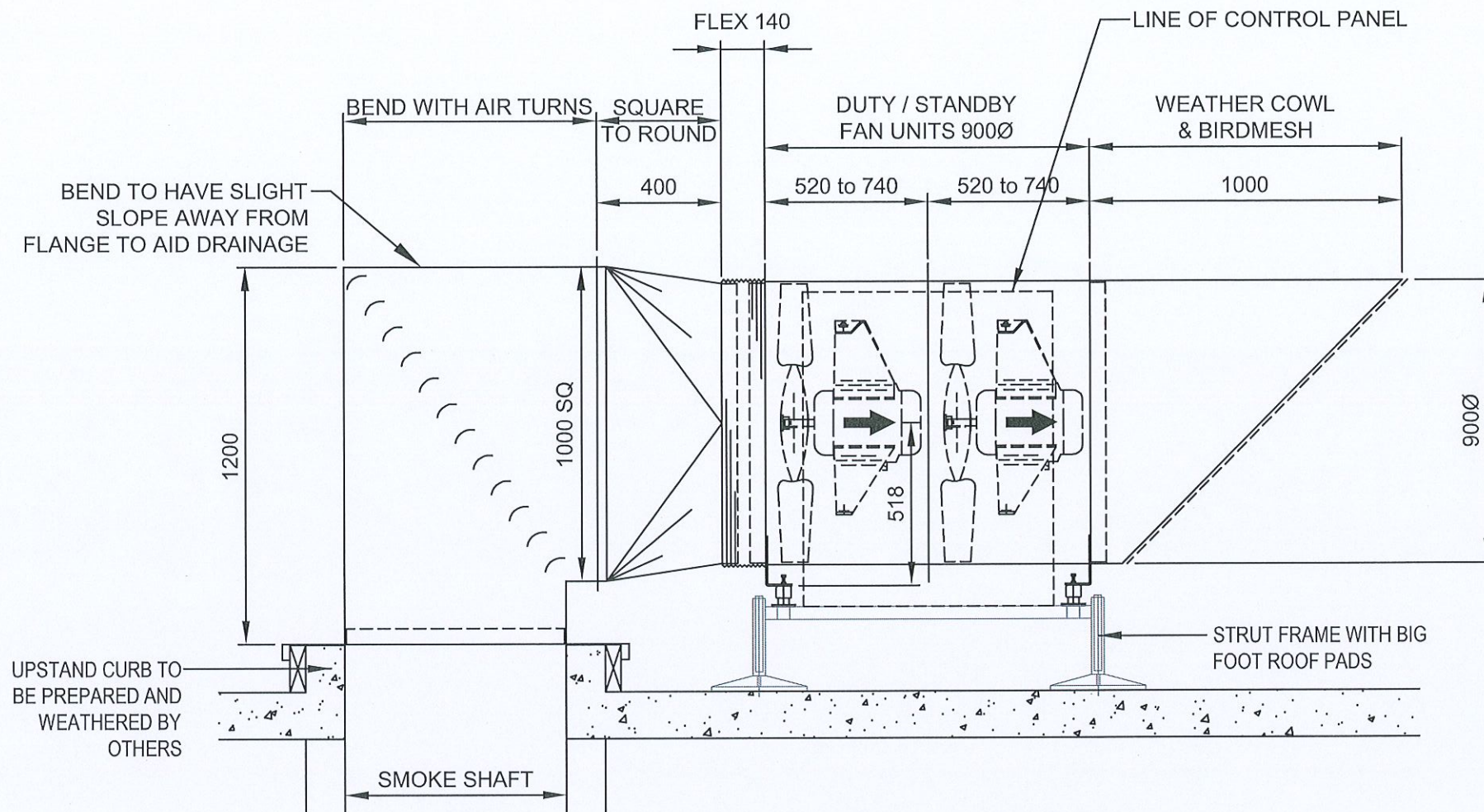
SIDE ELEVATION ON SMOKE FANS
