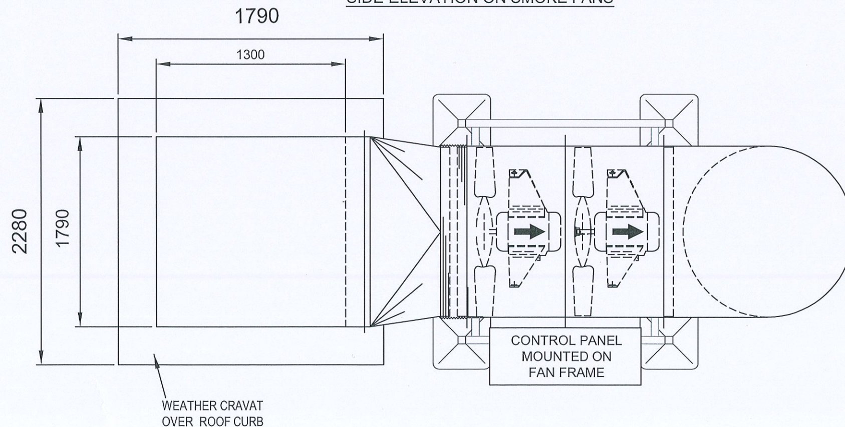
PLAN VIEW ON SMOKE FANS
