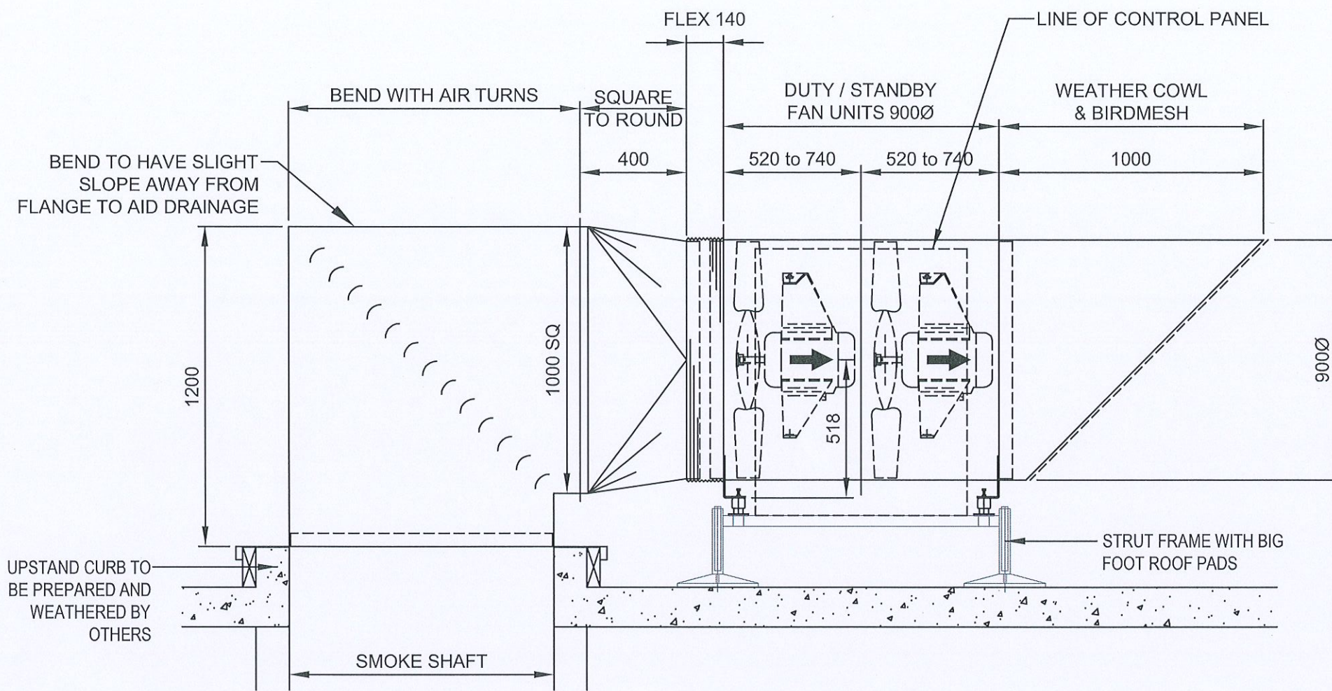
SIDE ELEVATION ON SMOKE FANS
