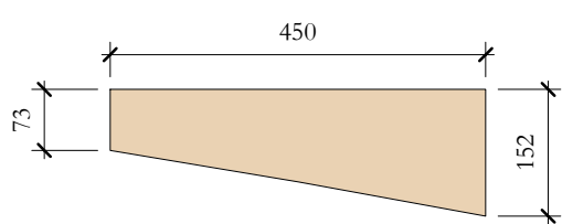
TcR_40 Elevation Front
