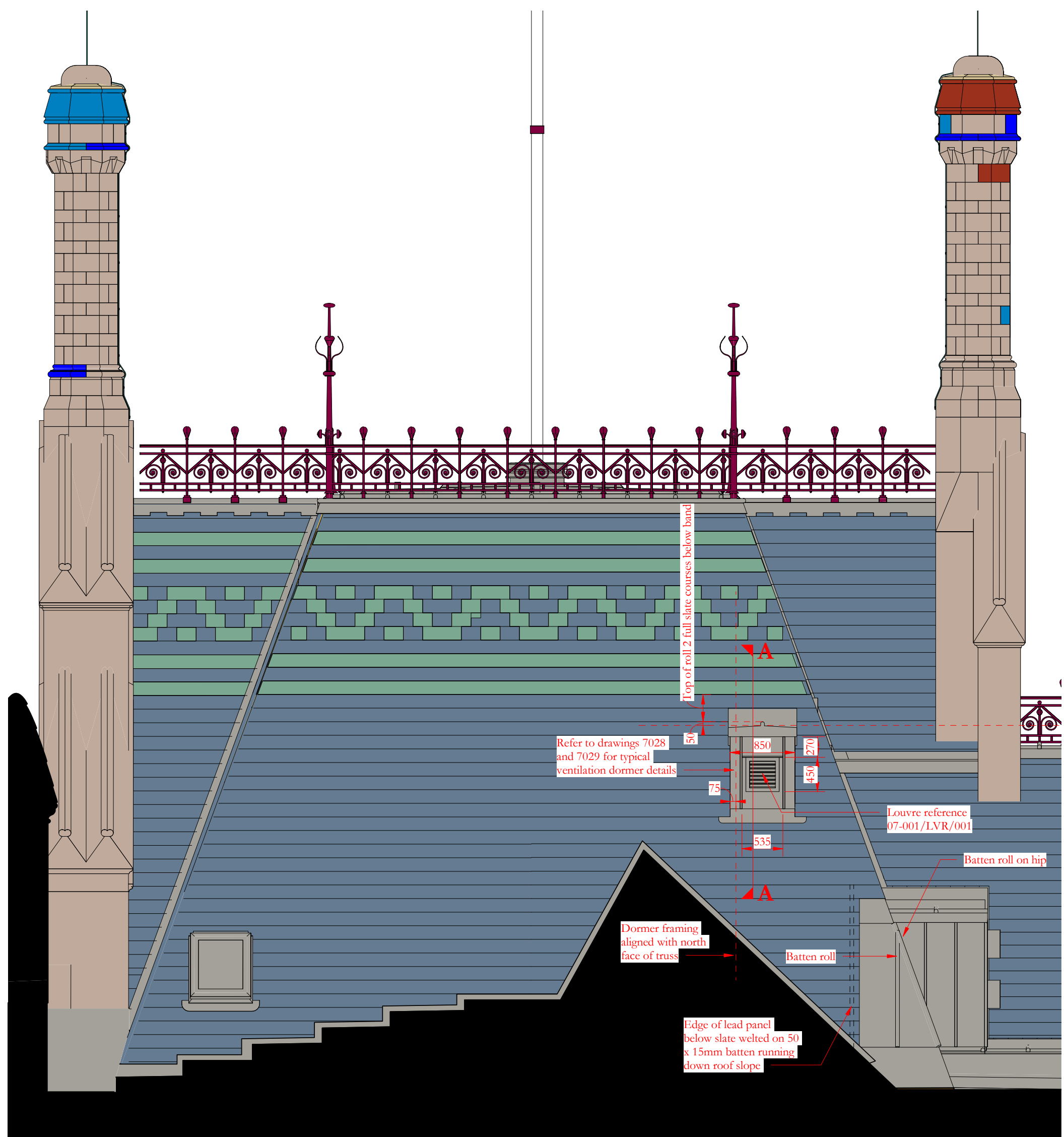
Elevation of roof slope WR22
