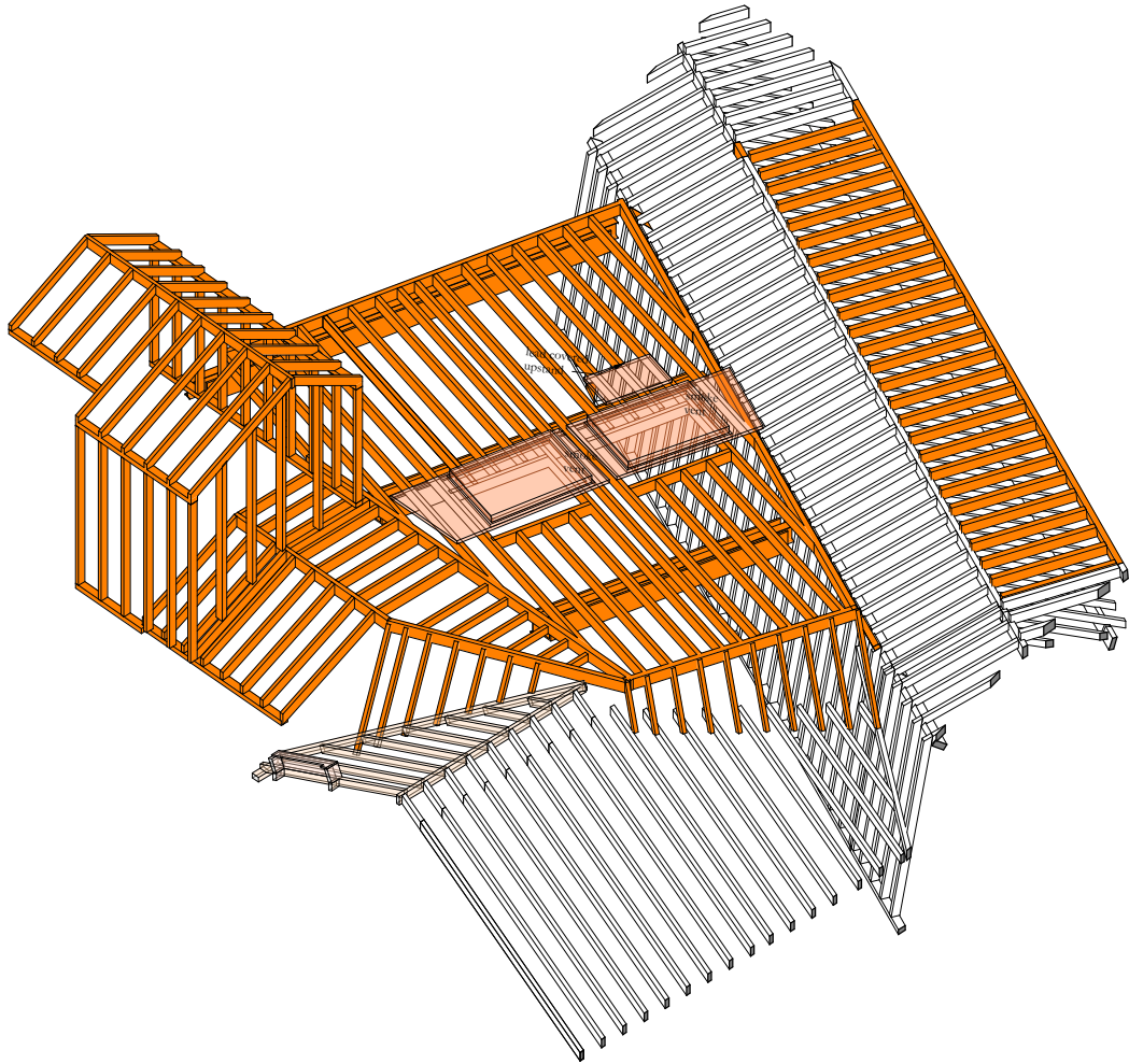
5b 3D View Area 5 - Structure Only
