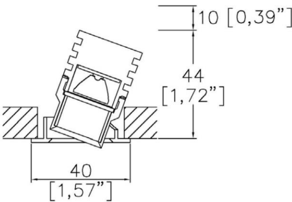
043-FA-TR Cut-out 36mm Ø
