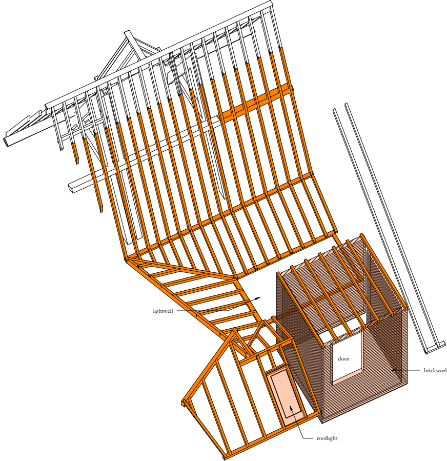
2b 3D View Area 2 - Structure Only
