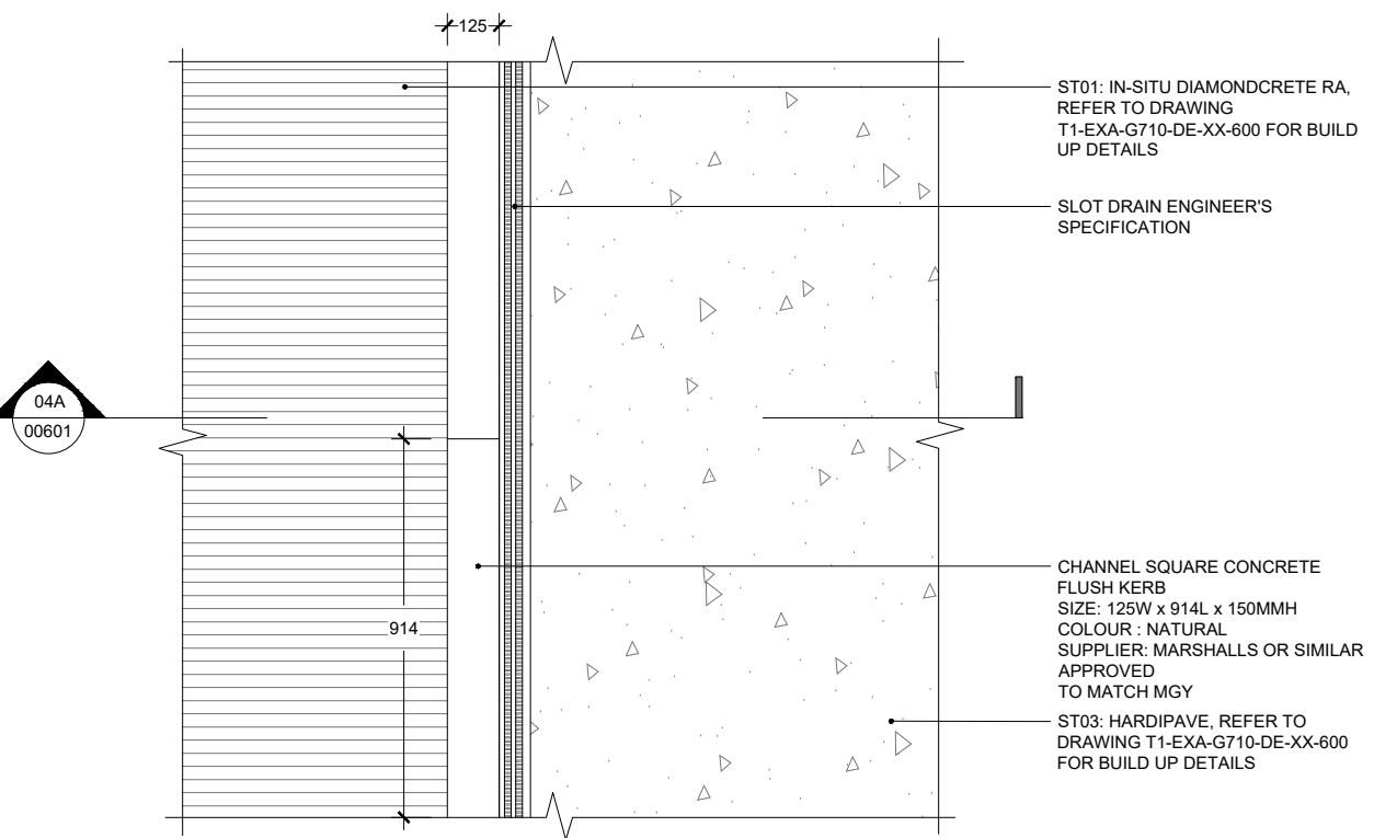
SLOT DRAIN AGAINST FLUSH KERB & HARDPAVE PLAN
