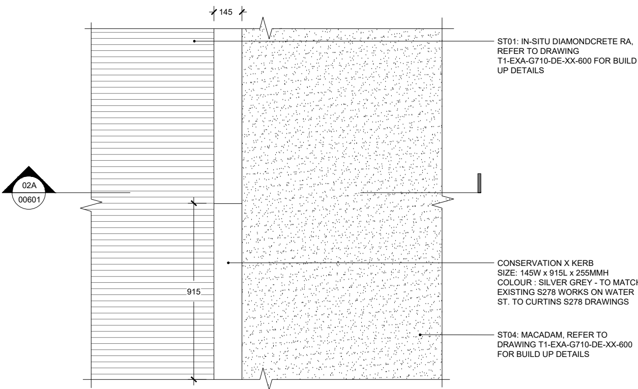
ET01: CONSERVATION X KERB IN-SITU DIAMONDCRETE 125MM DROP TO MACADAM PLAN
