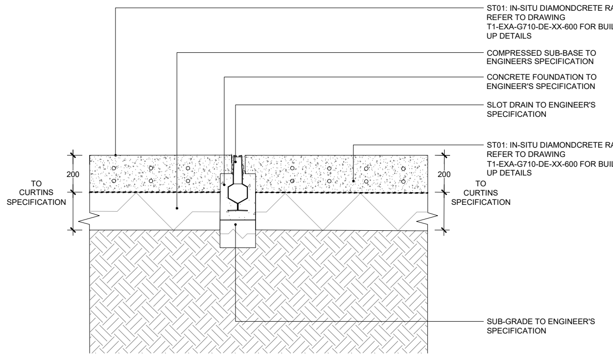
ET03: SLOT DRAIN IN DIAMONDCRETE RA SECTION
