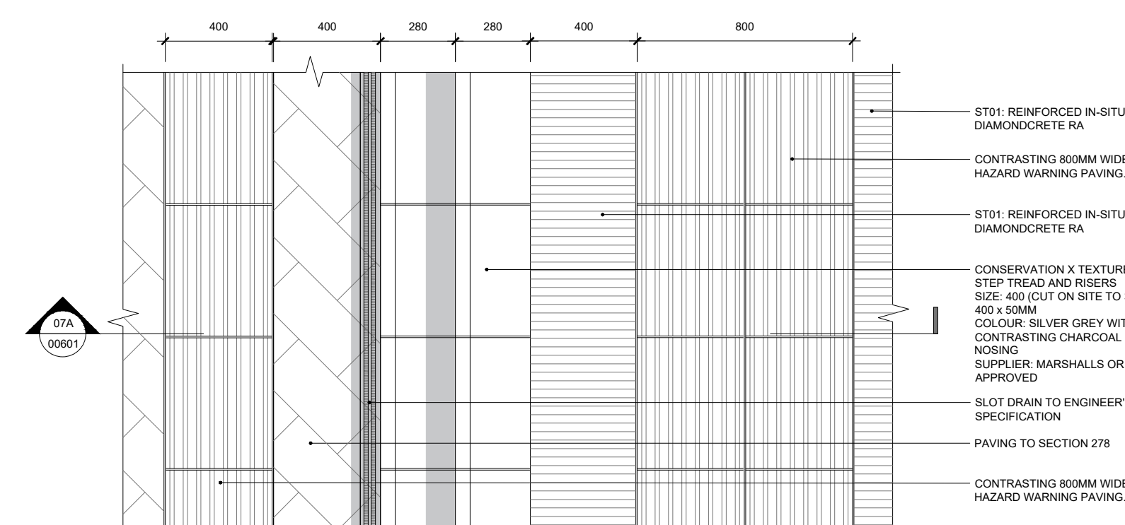
ET07A: STEPS PLAN
