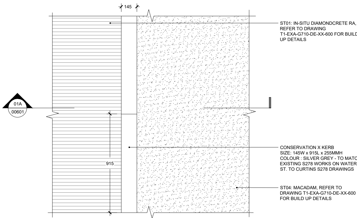
ET01: CONSERVATION X KERB IN-SITU DIAMONDCRETE 6MM DROP TO MACADAM PLAN
