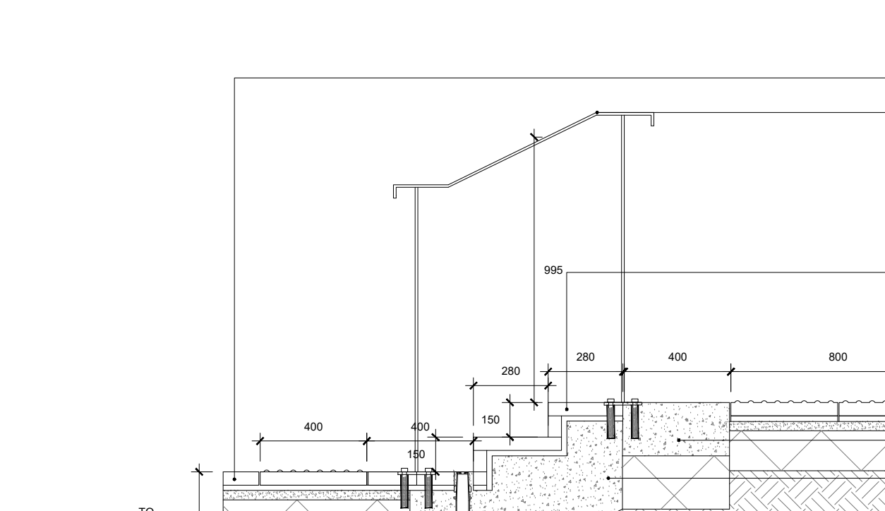
ET07A: STEPS SECTION
