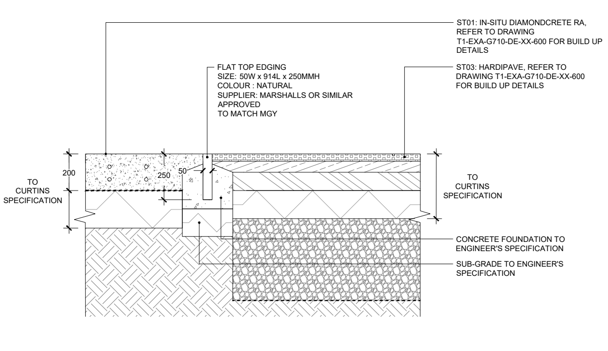
ET04: FLAT TOP EDGING AGAINST IN-SITU DIAMONDCRETE & HARDPAVE SECTION
