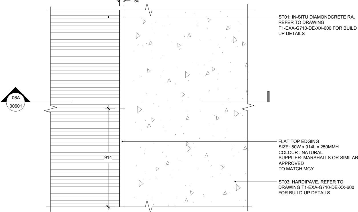
ET04: FLAT TOP EDGING AGAINST IN-SITU DIAMONDCRETE & HARDPAVE PLAN
