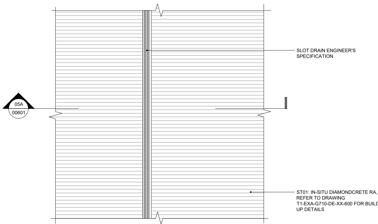
ET03: SLOT DRAIN IN DIAMONDCRETE RA PLAN
