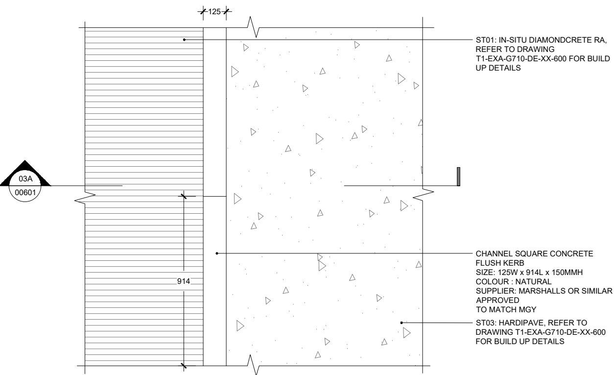
ET02: FLUSH KERB AGAINST IN-SITU DIAMONDCRETE & HARDPAVE PLAN
