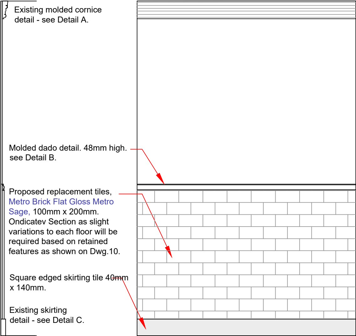
Section as Proposed:
