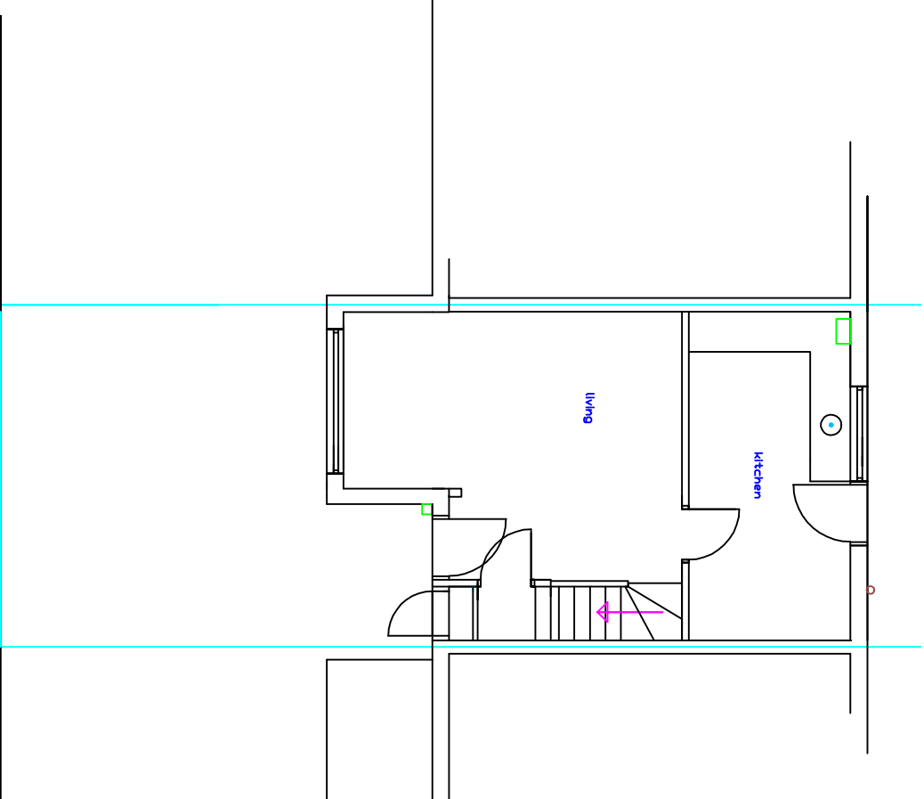
EXISTING GROUND FLOOR 1 : 100
