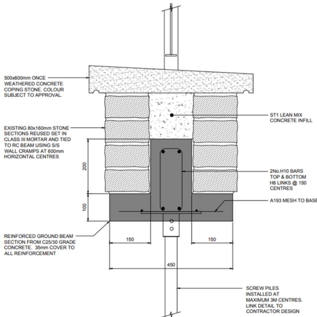
DETAIL 3 NORTH BOUNDARY FENCE AT SCREW PILE LOCATION
