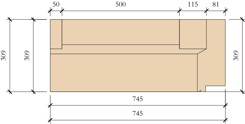
TcP_18 Elevation Front 1 : 10
