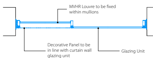
Plan Detail - Panel D
