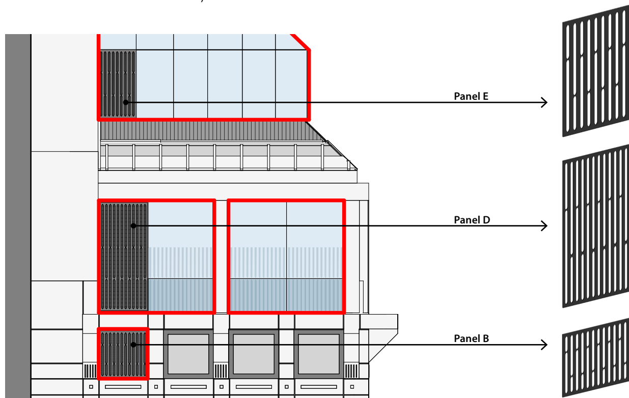
Close Up North Elevation - Barnett House
