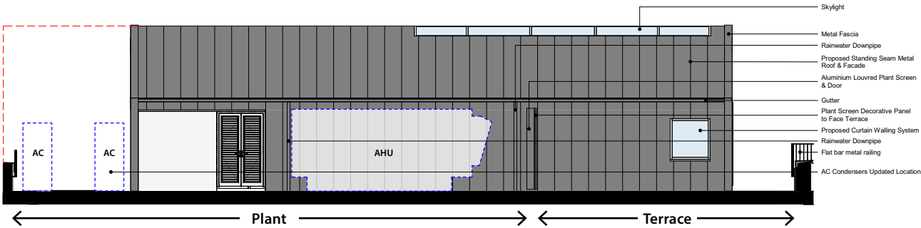
Proposed West Elevation - Fountain Street
