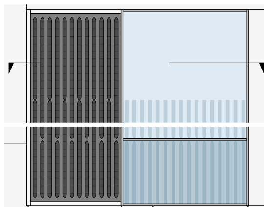
Elevation Detail - Panel D
