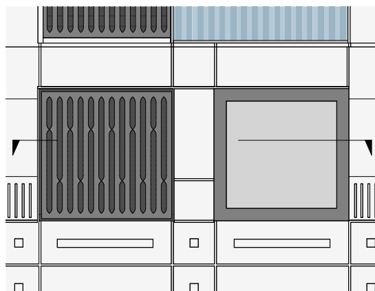
Elevation Detail - Panel B
