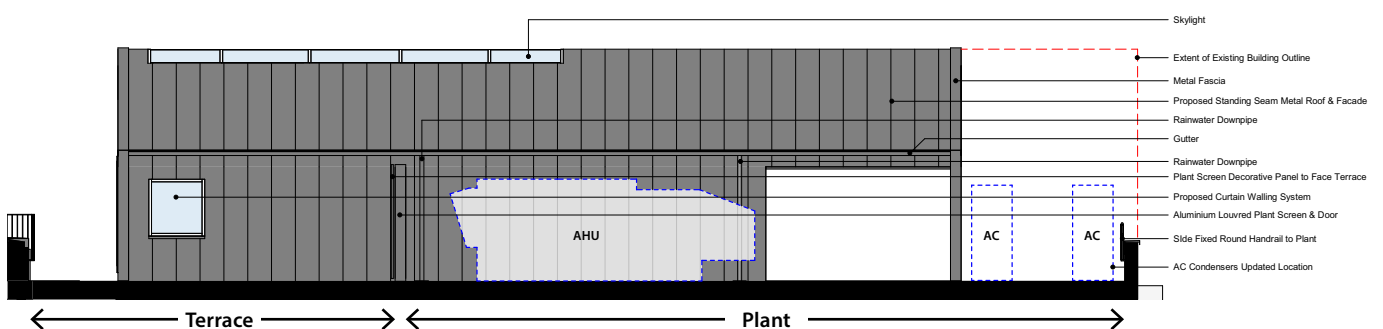
Proposed East Elevation - West Mosley Street
