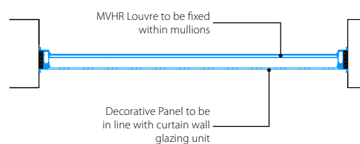
Plan Detail - Panel C
