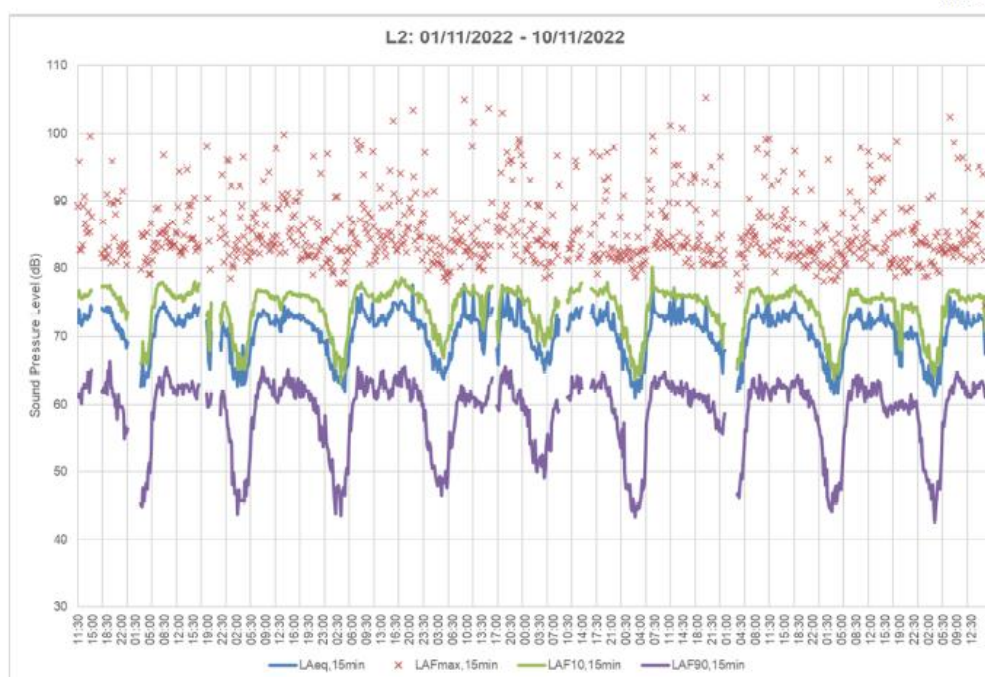
Figure C2 – Buro Happold graphed noise data, measurement position L2
