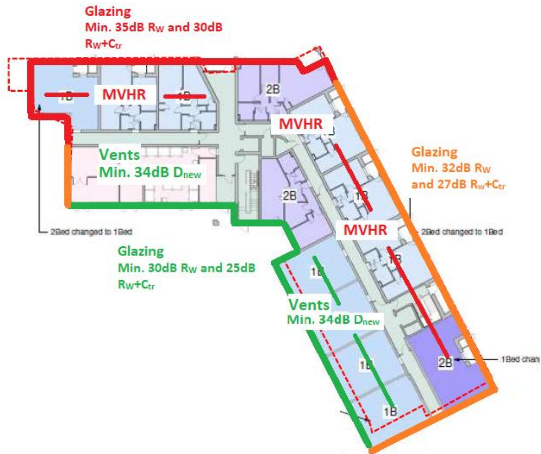
Figure 13 – Glazing and Ventilation Specification for all facades and all floor levels.
