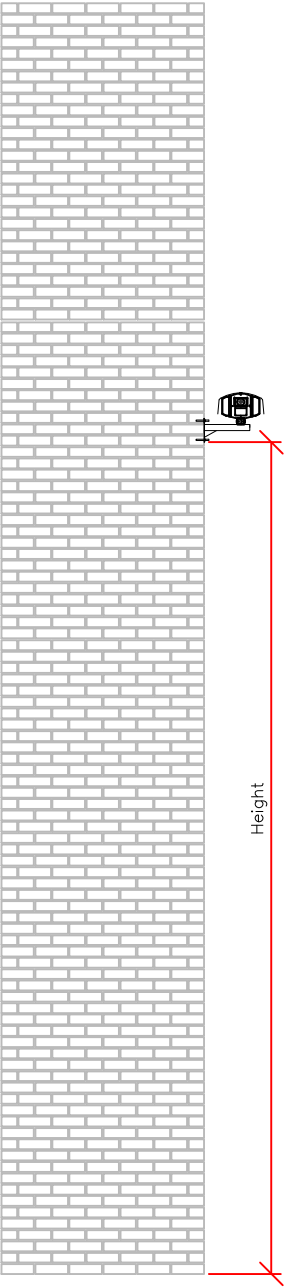
Camera General Arrangement Detail SIDE ELEVATION
