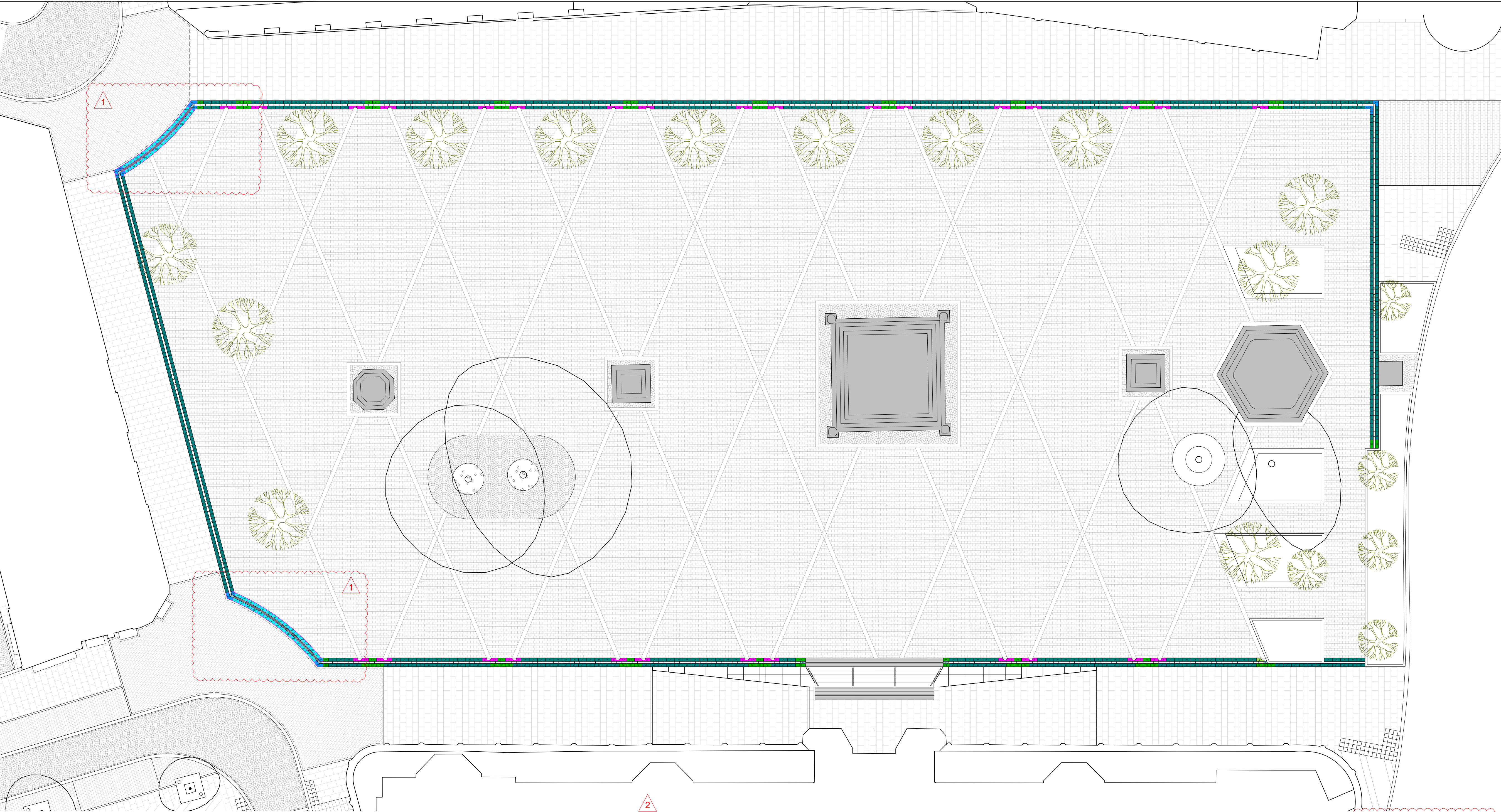
Paving Schedule - Granite Perimeter Paving Channel - REF S2.3
