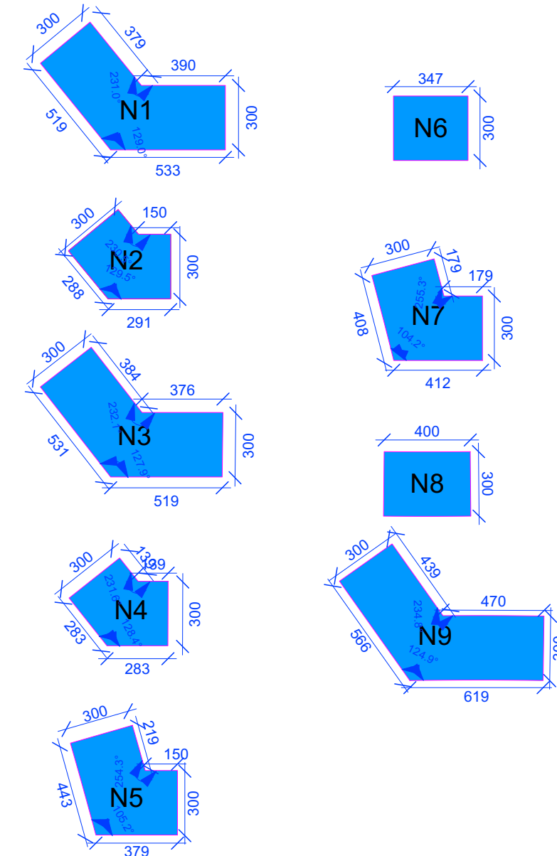
5 Perimeter Channel Corner Units Scale: 1:25
