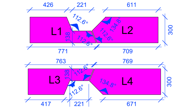
3 Intersection unit - Diamond Band Scale: 1:25
