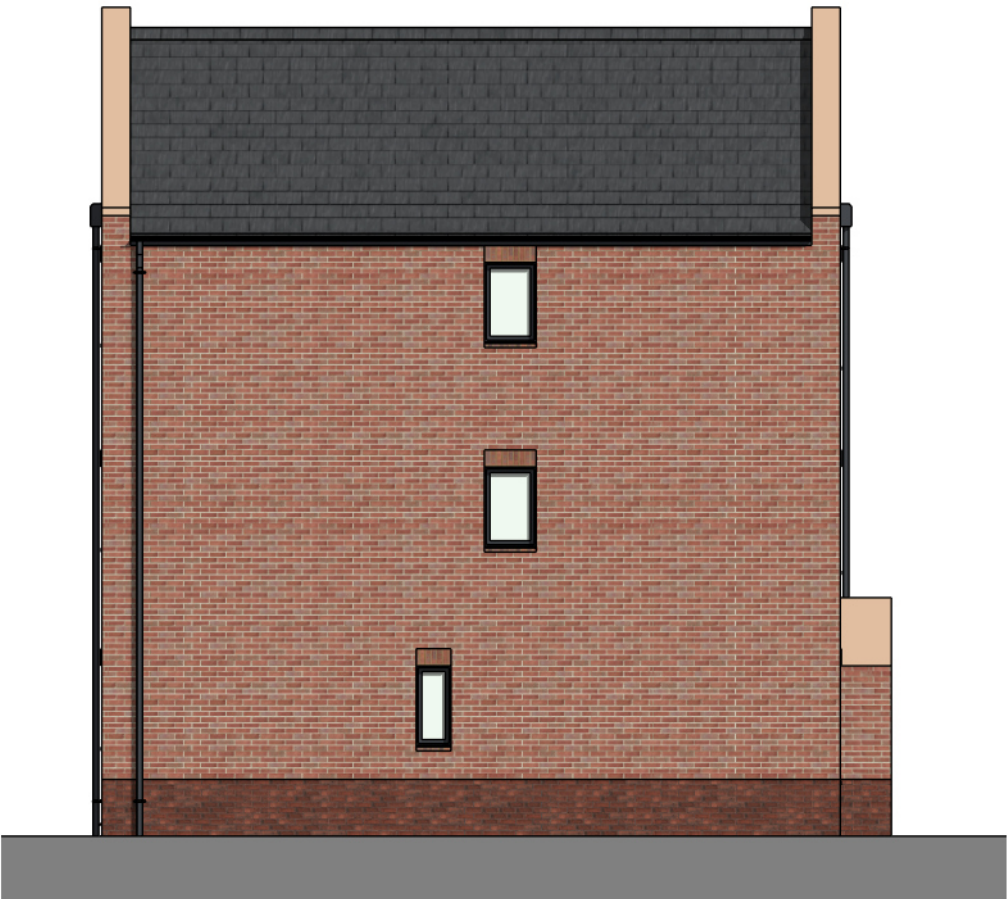
Left Elevation 1 : 100
