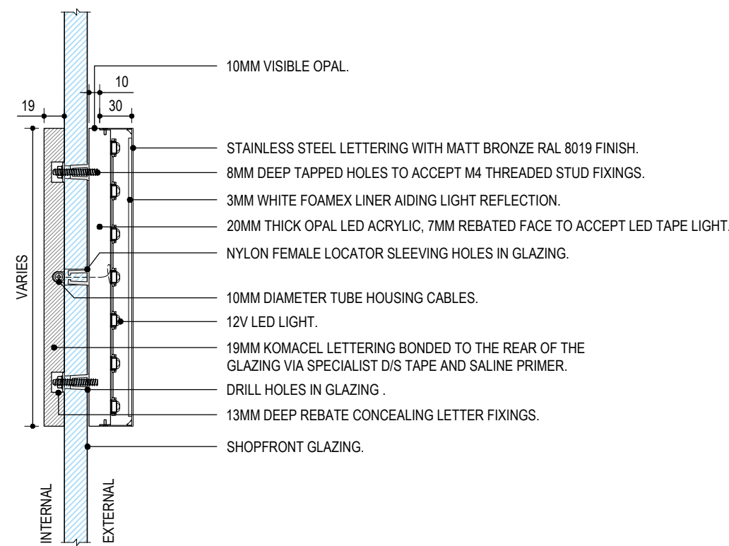
03 PROPOSED SIGNAGE LETTERING SECTION DETAIL SCALE 1:5@A1; 1:10@A3
