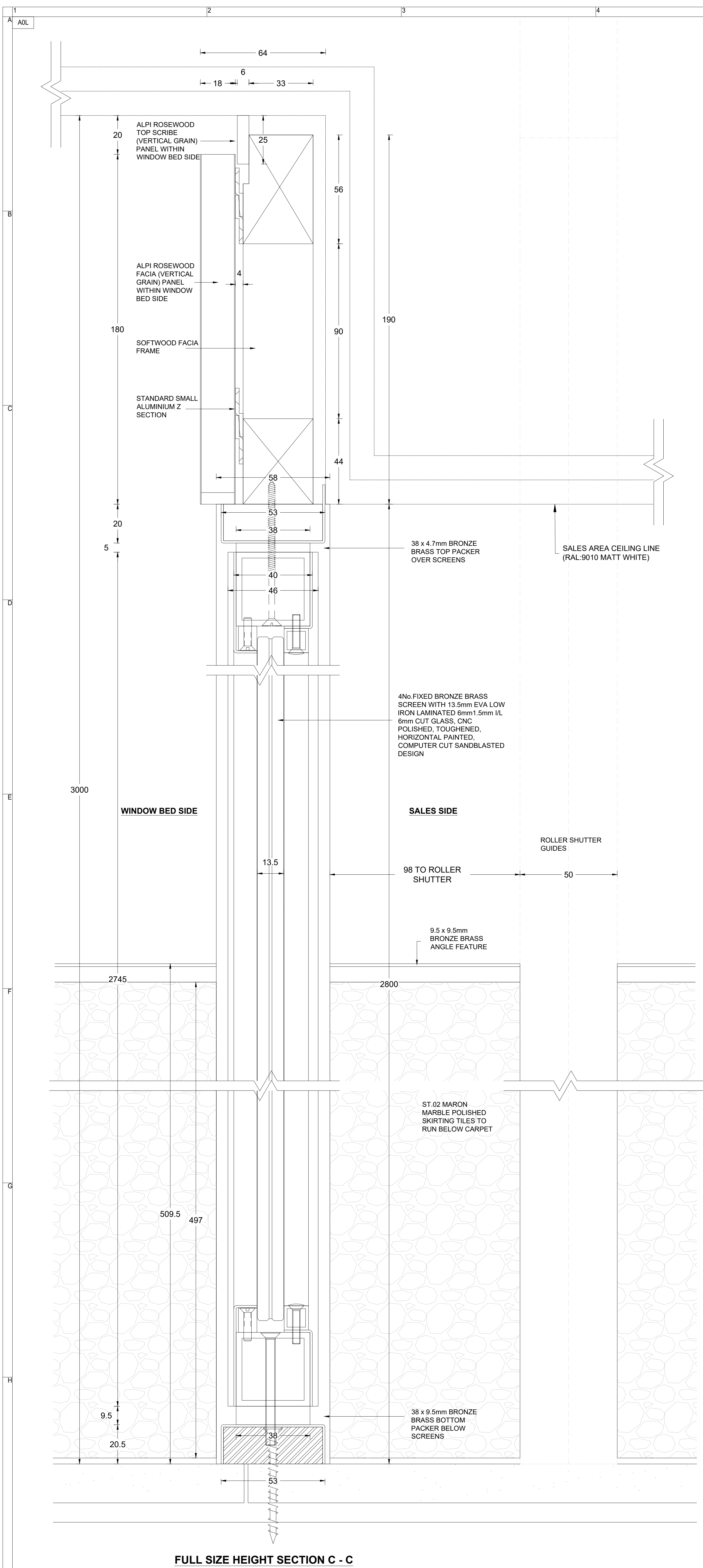
FULL SIZE HEIGHT SECTION C - C
