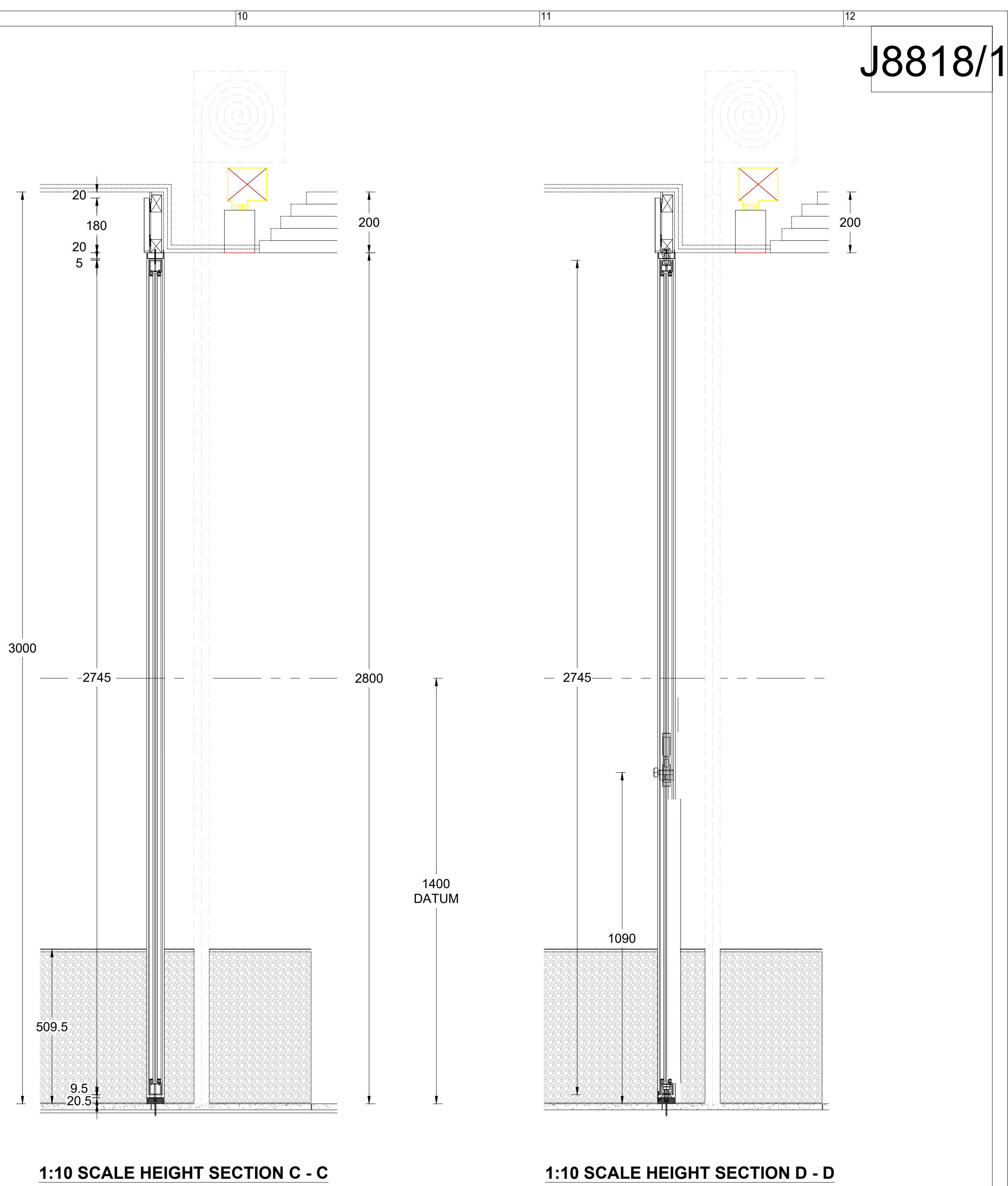
1:10 SCALE HEIGHT SECTION C - C
