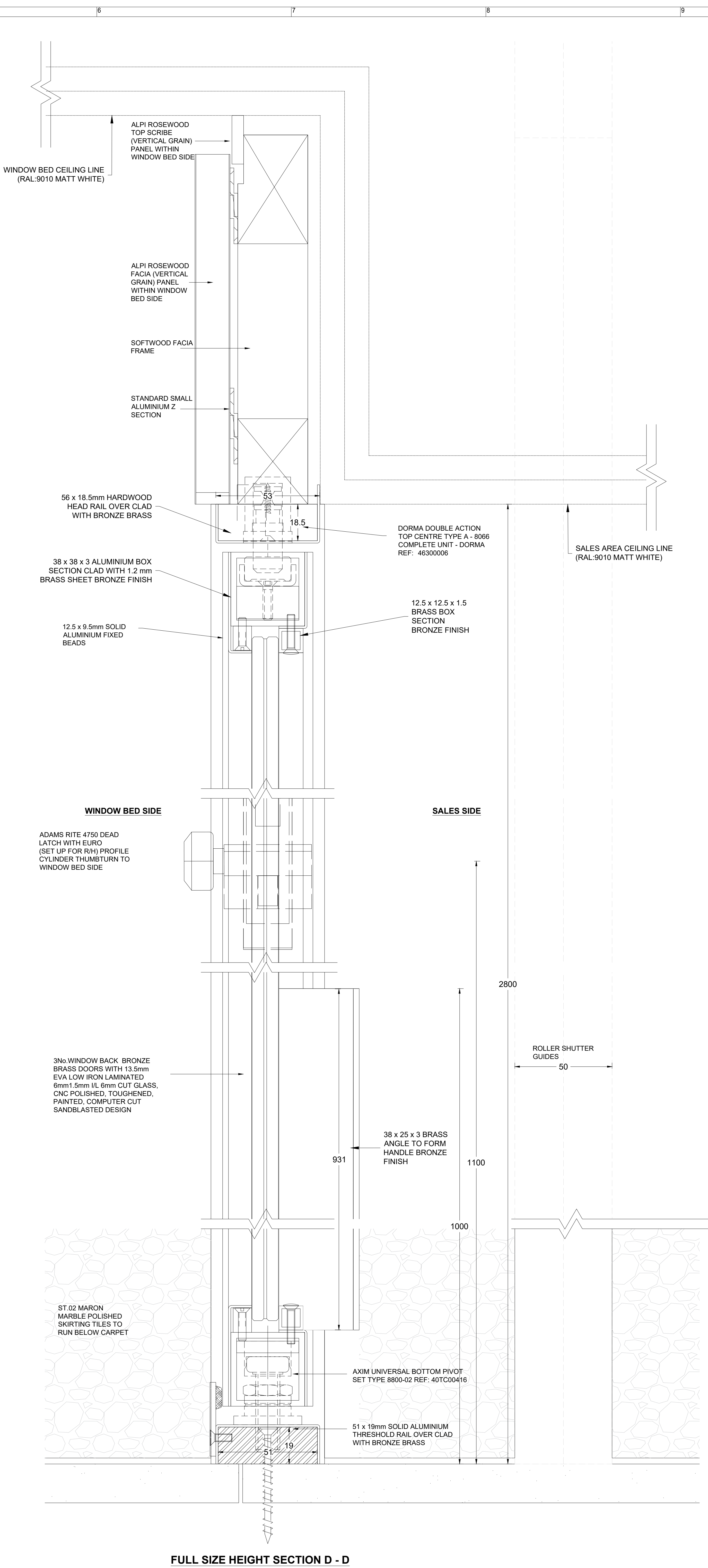
FULL SIZE HEIGHT SECTION D - D
