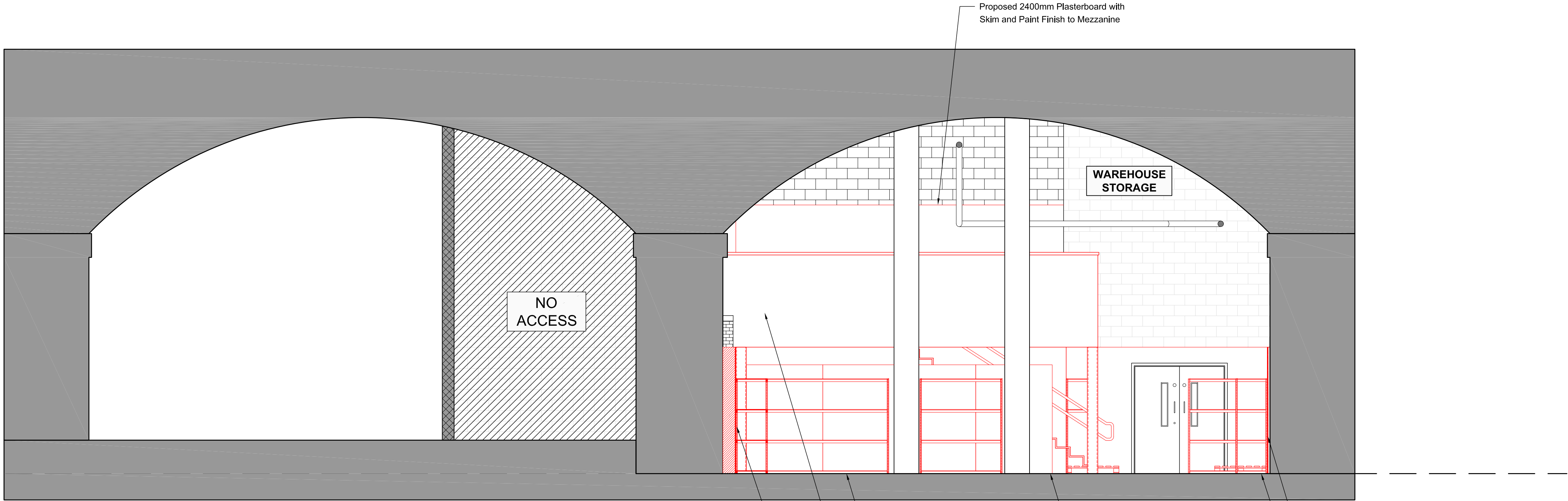
Proposed Section G-G Scale 1 : 50
