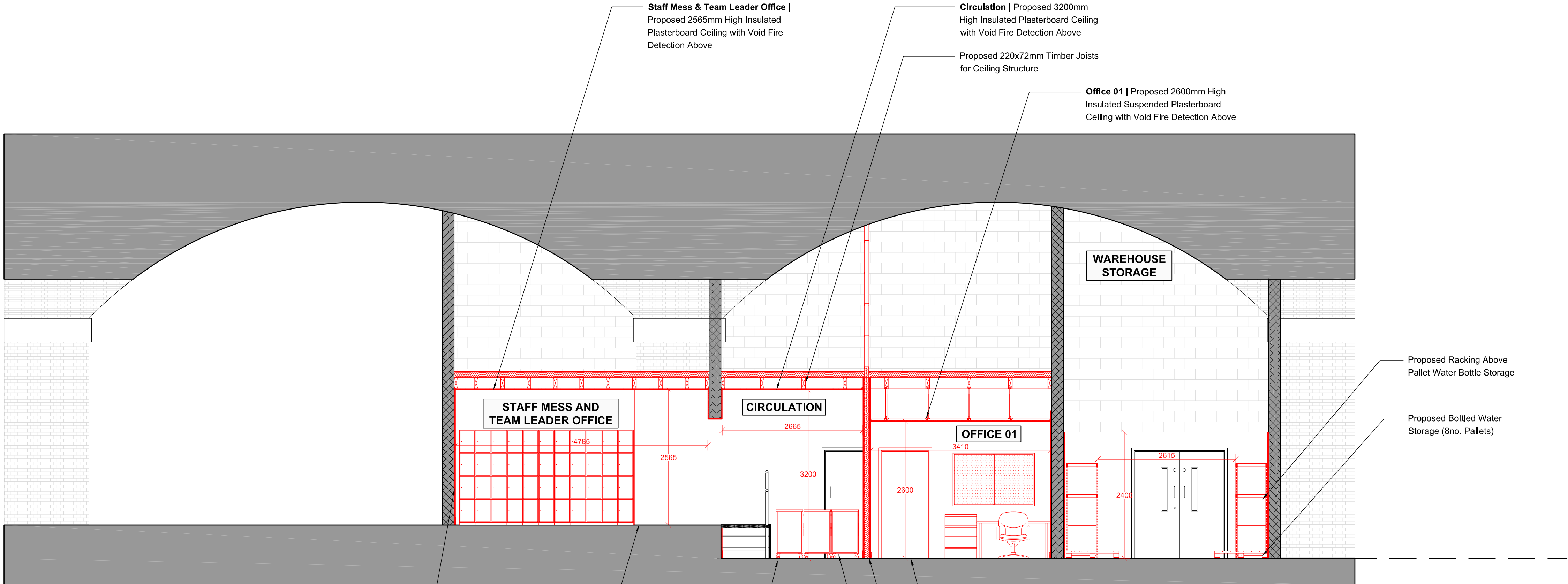
Proposed Section H-H Scale 1 : 50
