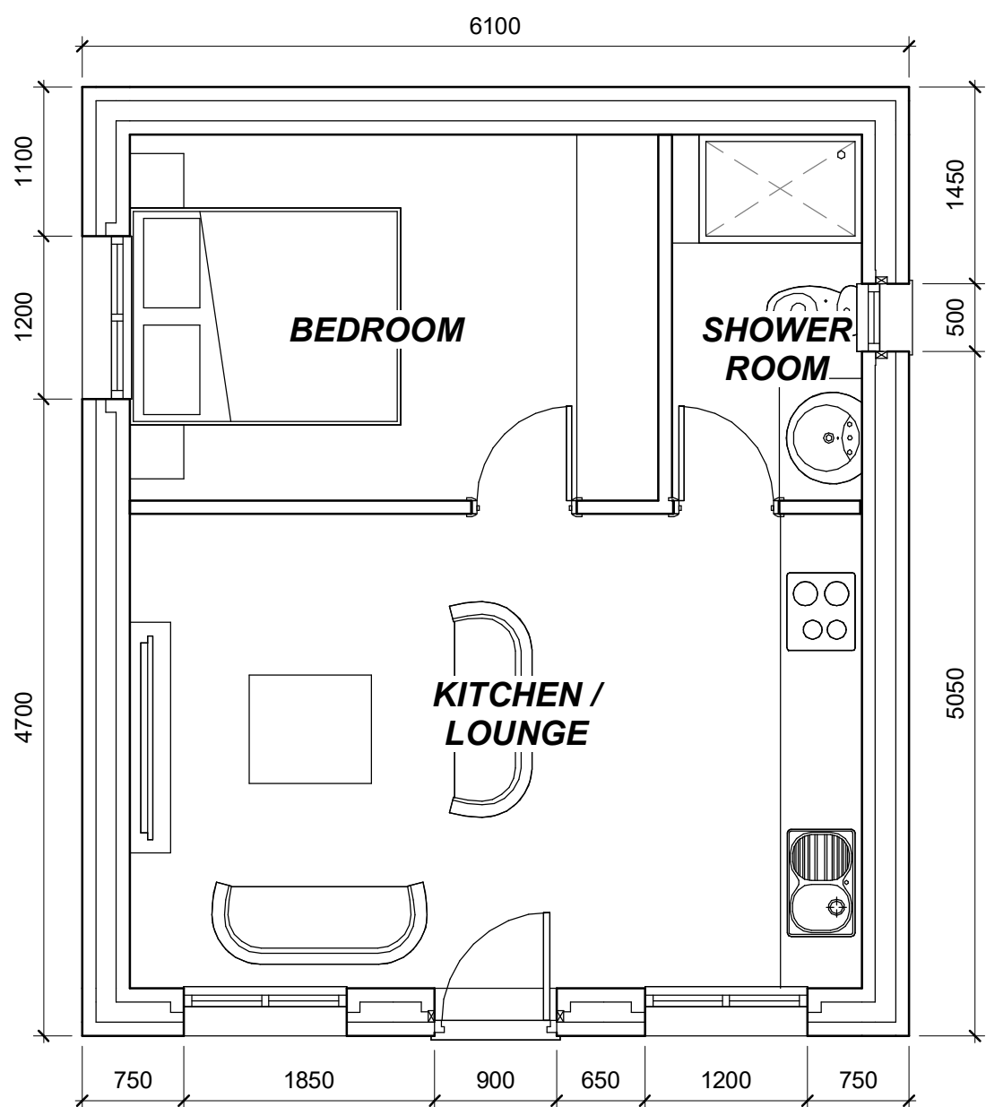
Proposed Ground Floor Layout (Outbuilding) 1 : 50
