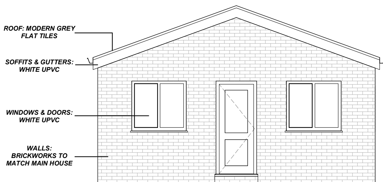
Proposed Elevation A (Outbuilding) 1 : 50
