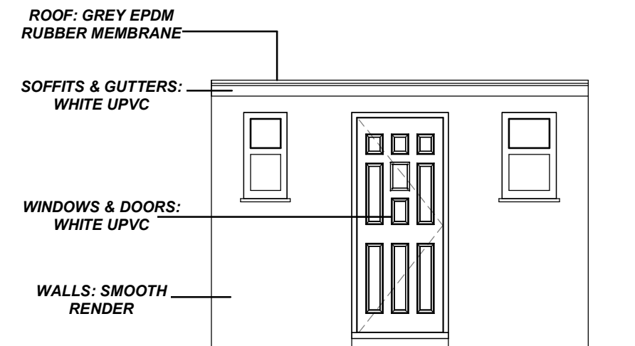
Proposed Elevation A (Shed) 1 : 50
