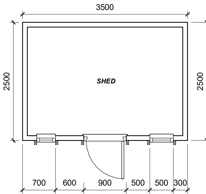
Proposed Ground Floor Layout (Shed) 1 : 50
