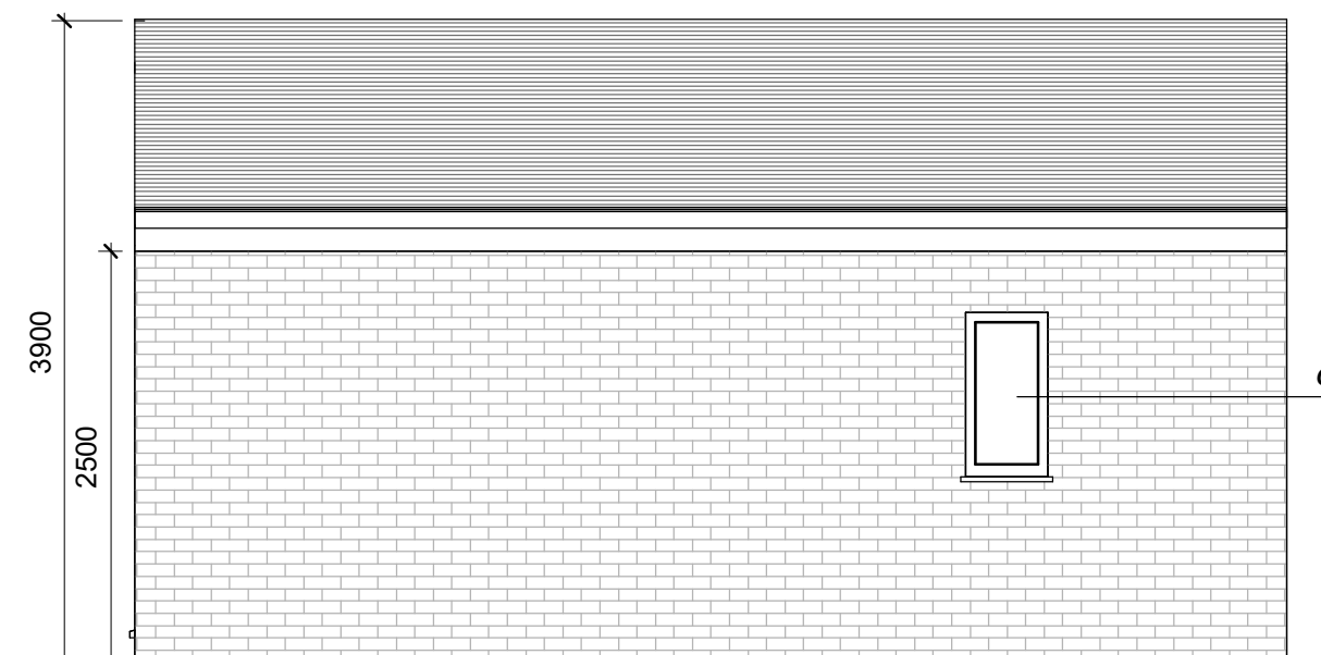
Proposed Elevation D (Outbuilding) 1 : 50
