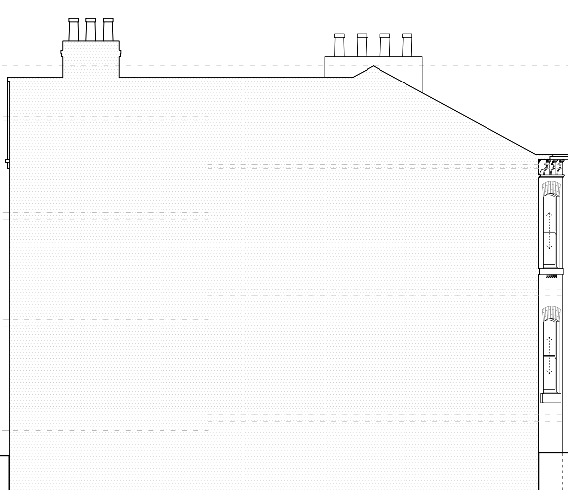
PROPOSED SIDE ELEVATION (PARTY WALL)
