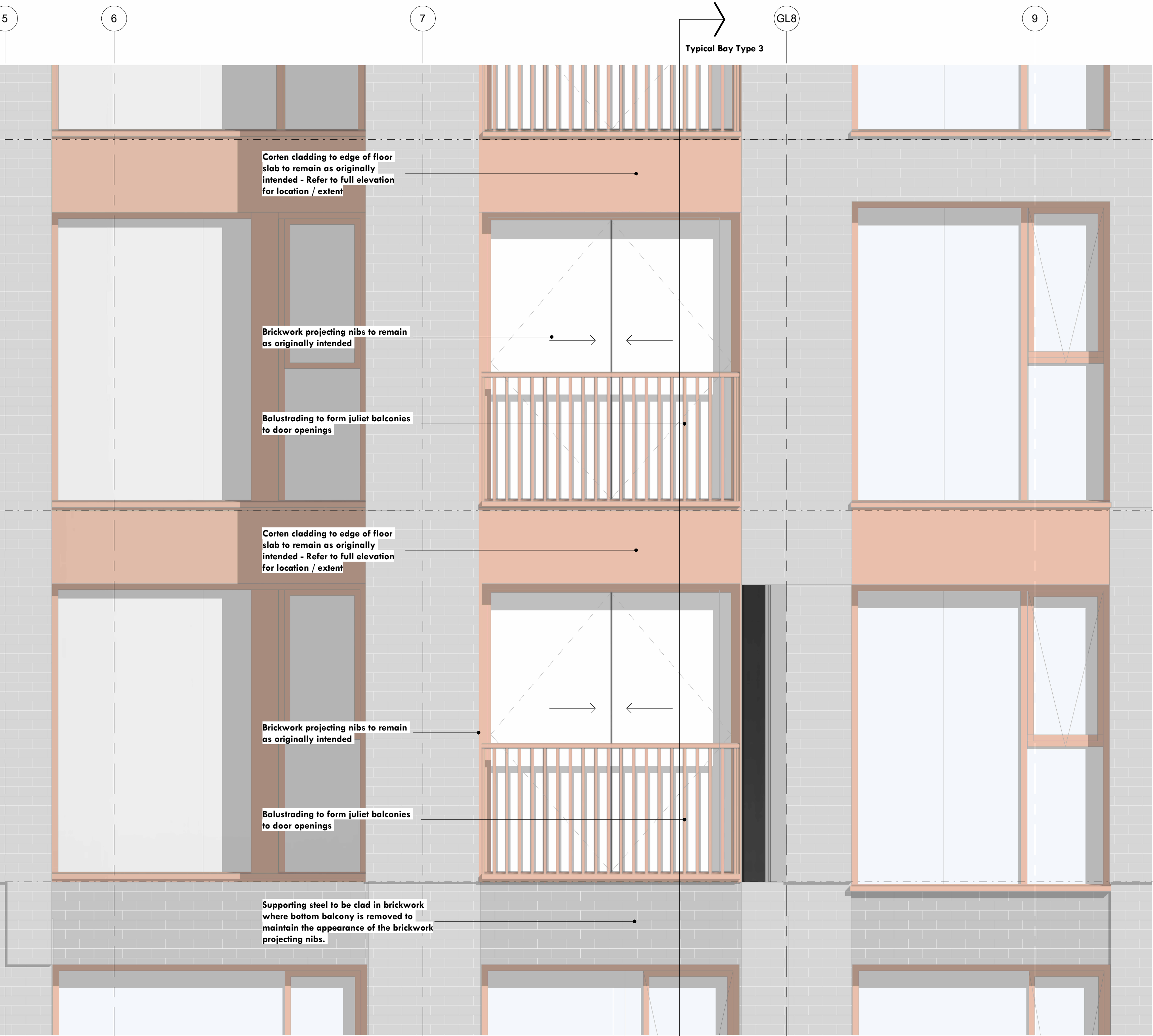
Typical Bays Elevation 1 : 20
