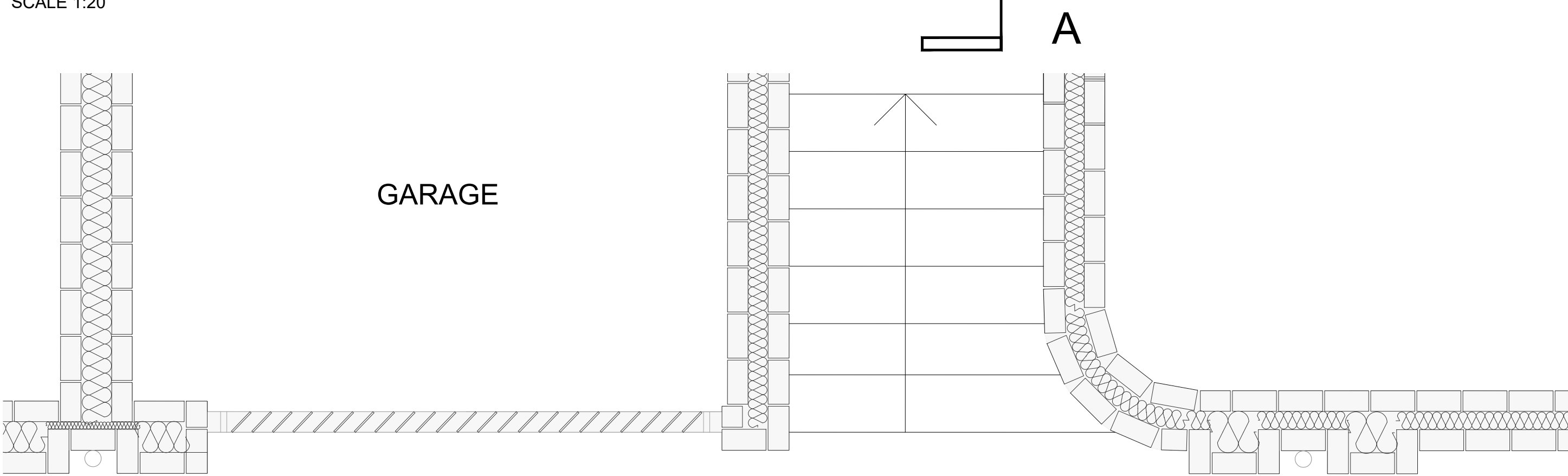
SECTION B:B SCALE 1:20
