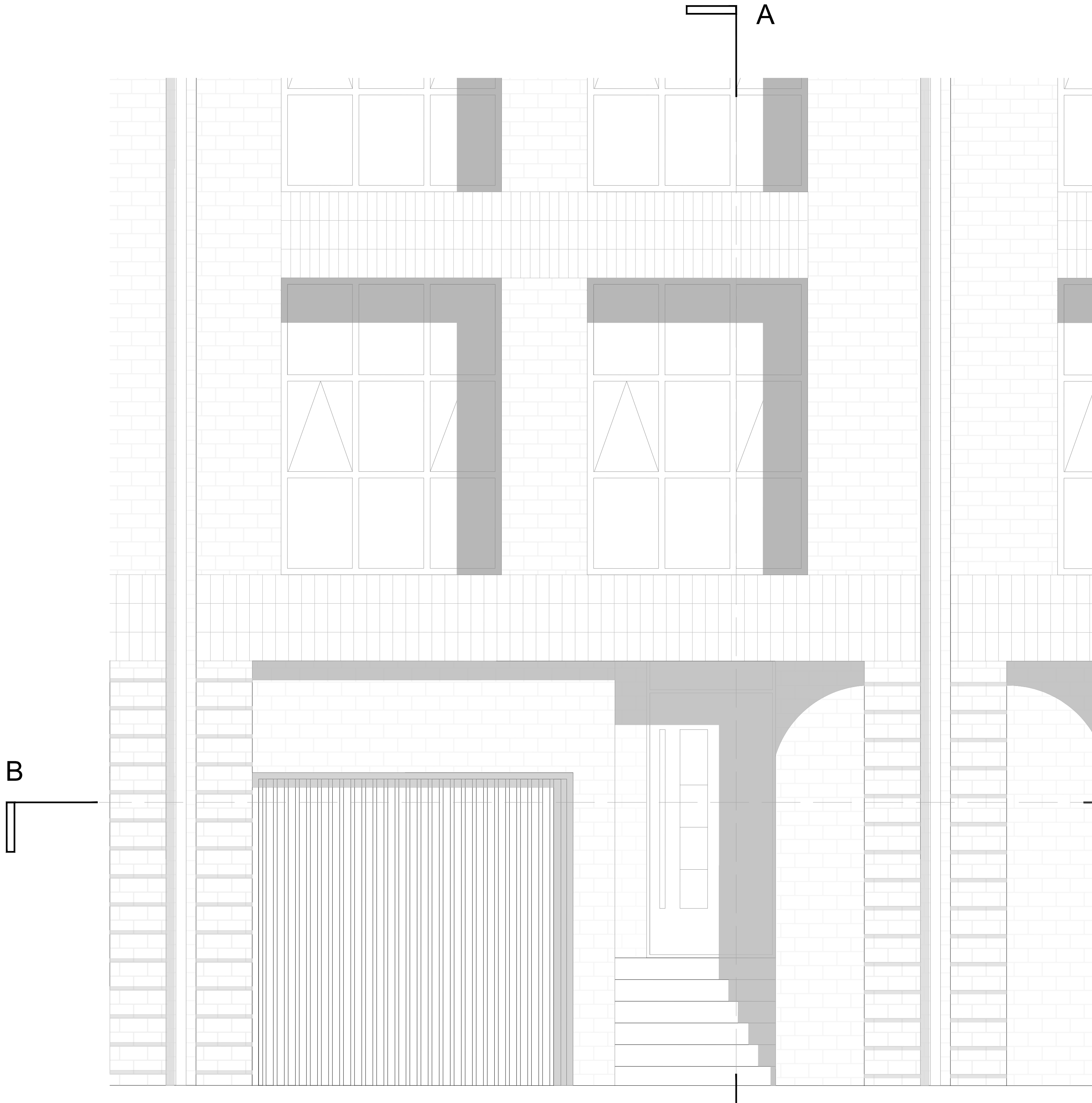
ELEVATION SCALE 1:20
