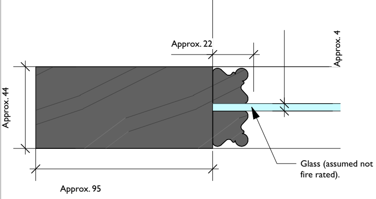
1 Door Section Detail - Through Glass Panel Scale: Half Actual Size
