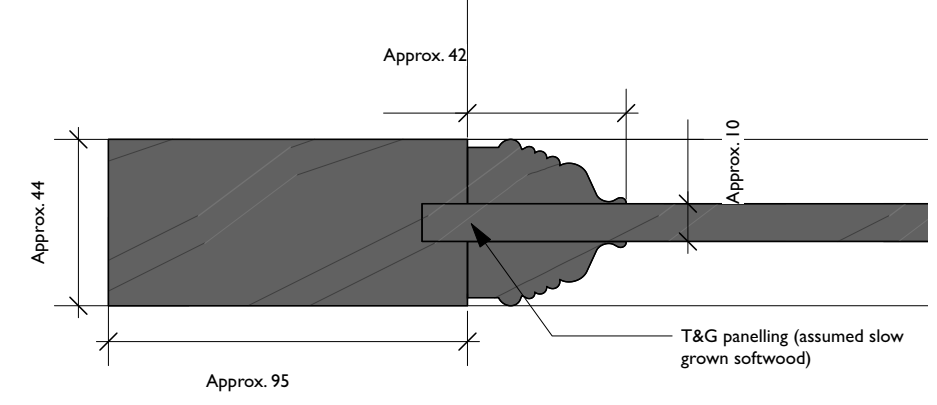
3 Door Section Detail - Through Thick Panel Scale: Half Actual Size
