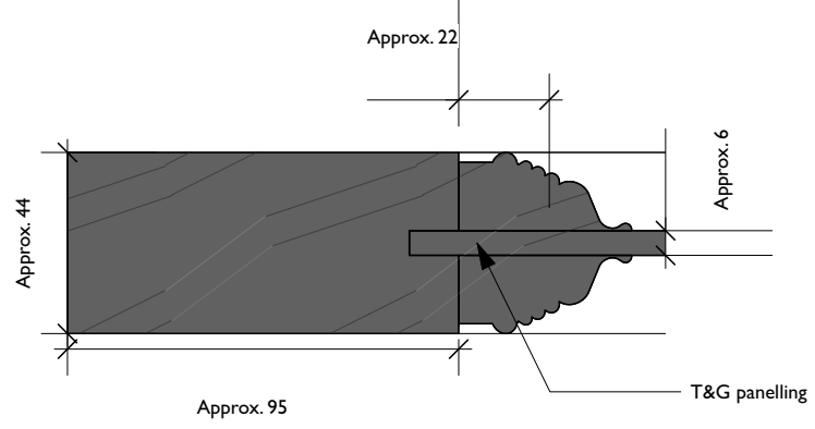
2 Door Section Detail - Through Thin Panel Scale: Half Actual Size
