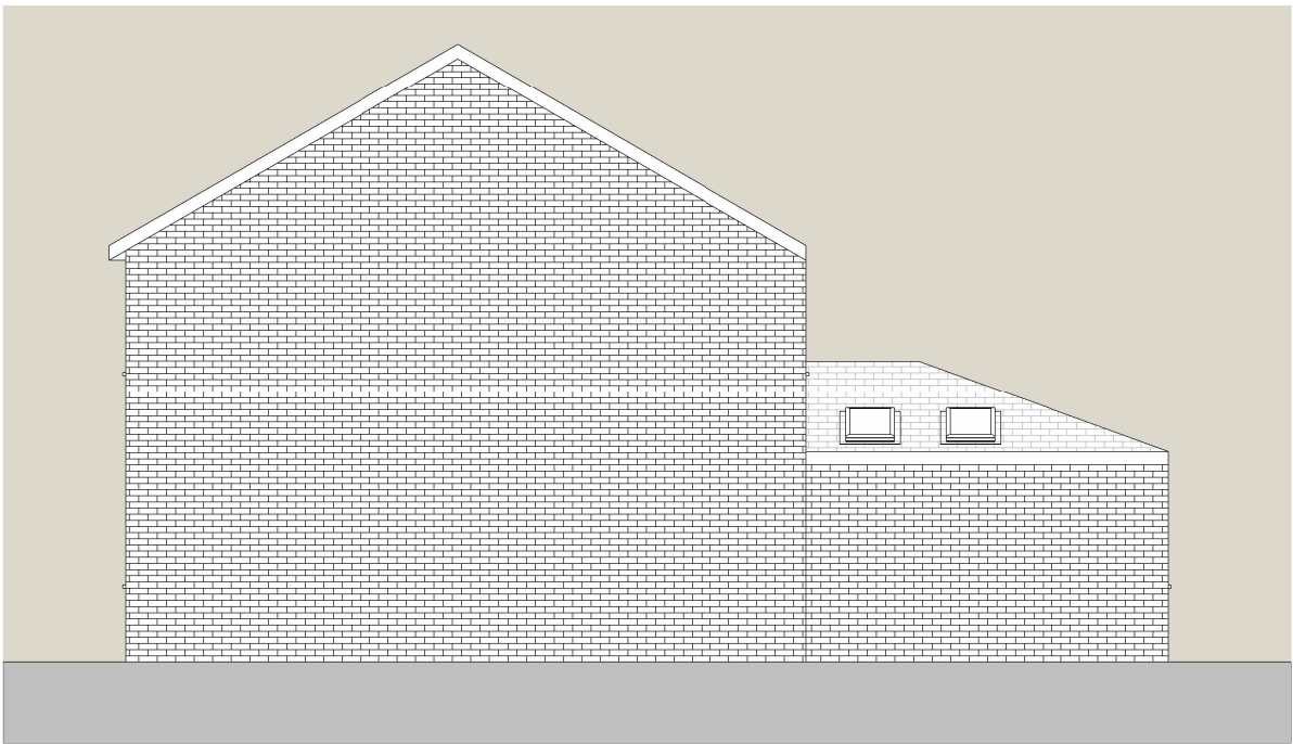
PP RHS Elevation 1 : 100
