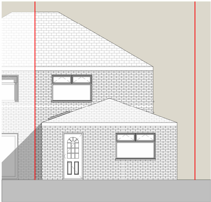
PP Rear Elevation 1 : 100
