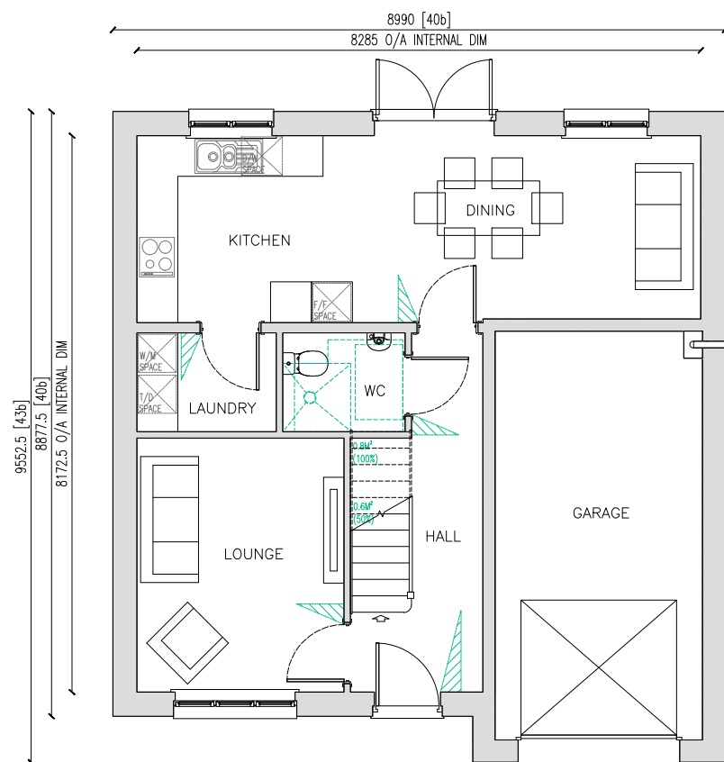
GROUND FLOOR GROSS INTERNAL AREA 50.18m 2
