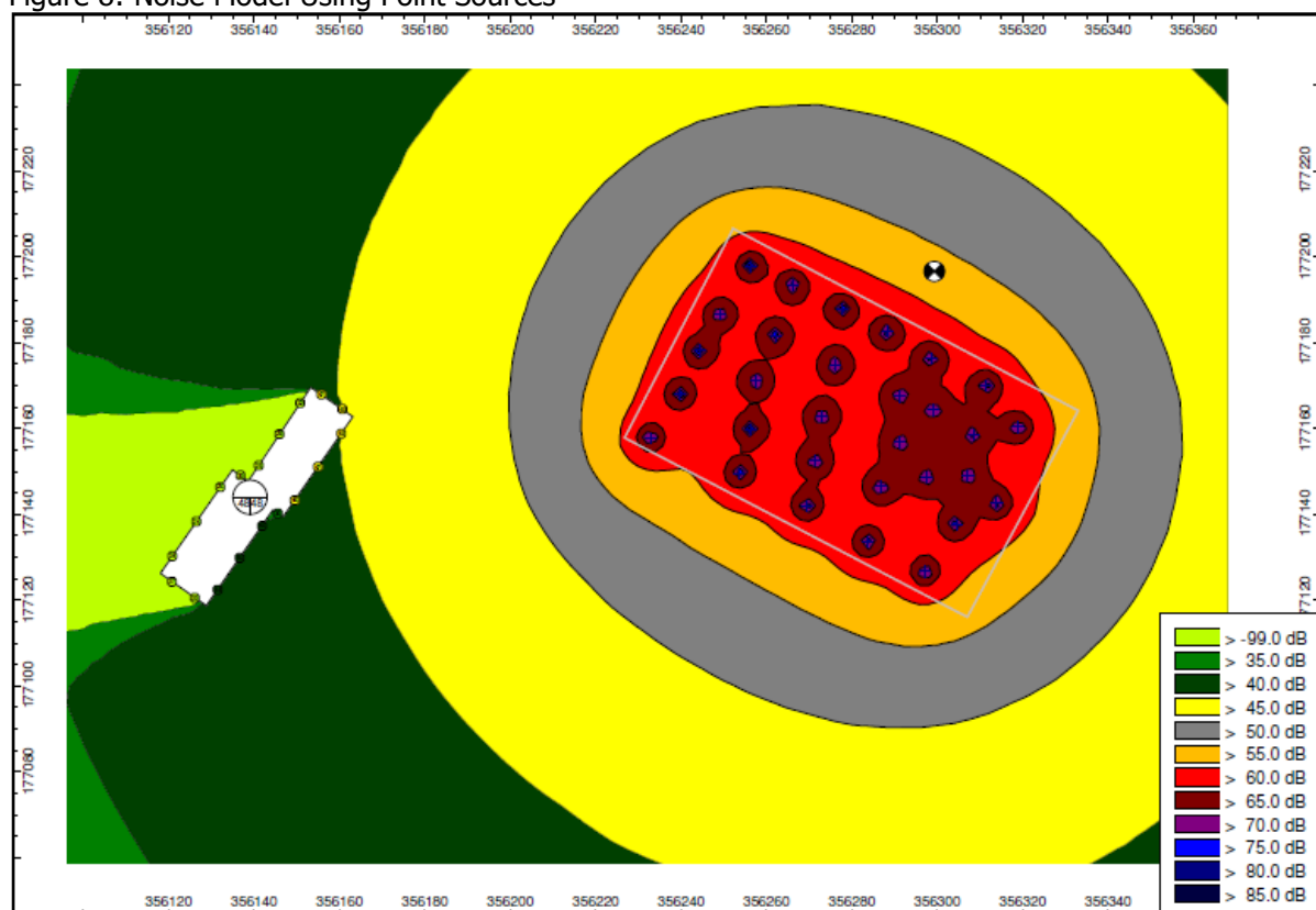
Figure 8: Noise Model Using Point Sources
