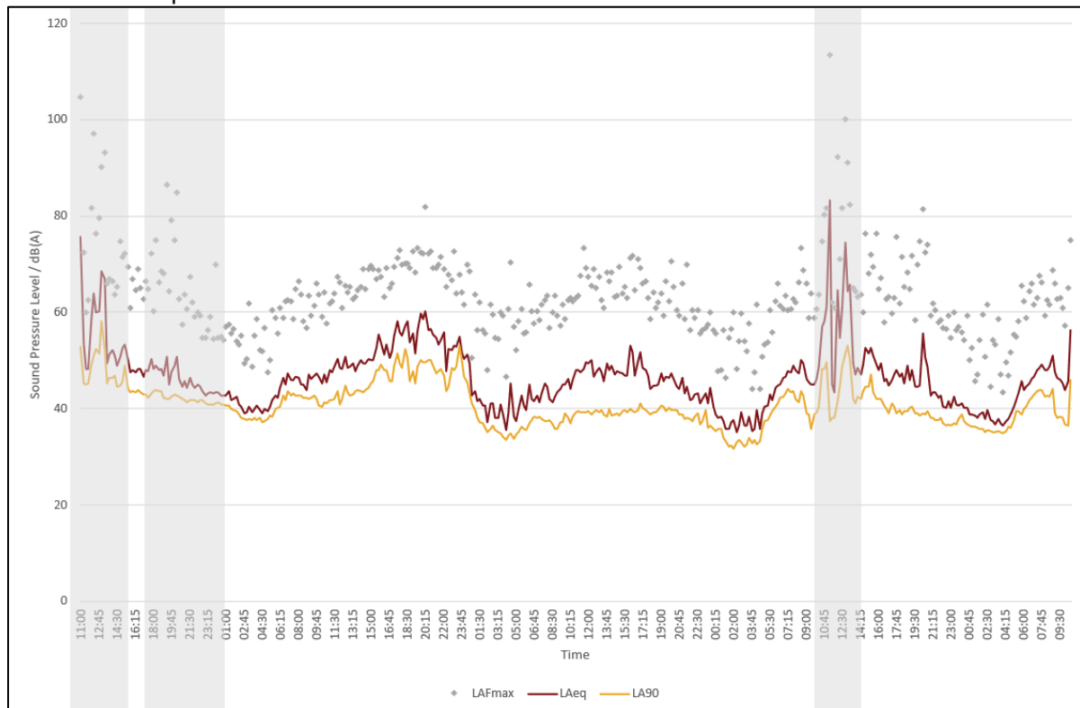
Figure 3: Measured noise levels at monitoring location over time (free-field), where the greyed out sections reflect periods of excluded data
