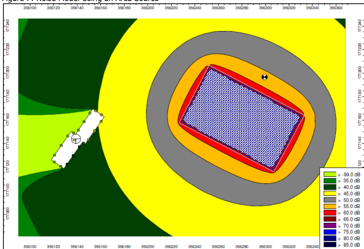
Figure 7: Noise Model Using an Area Source
