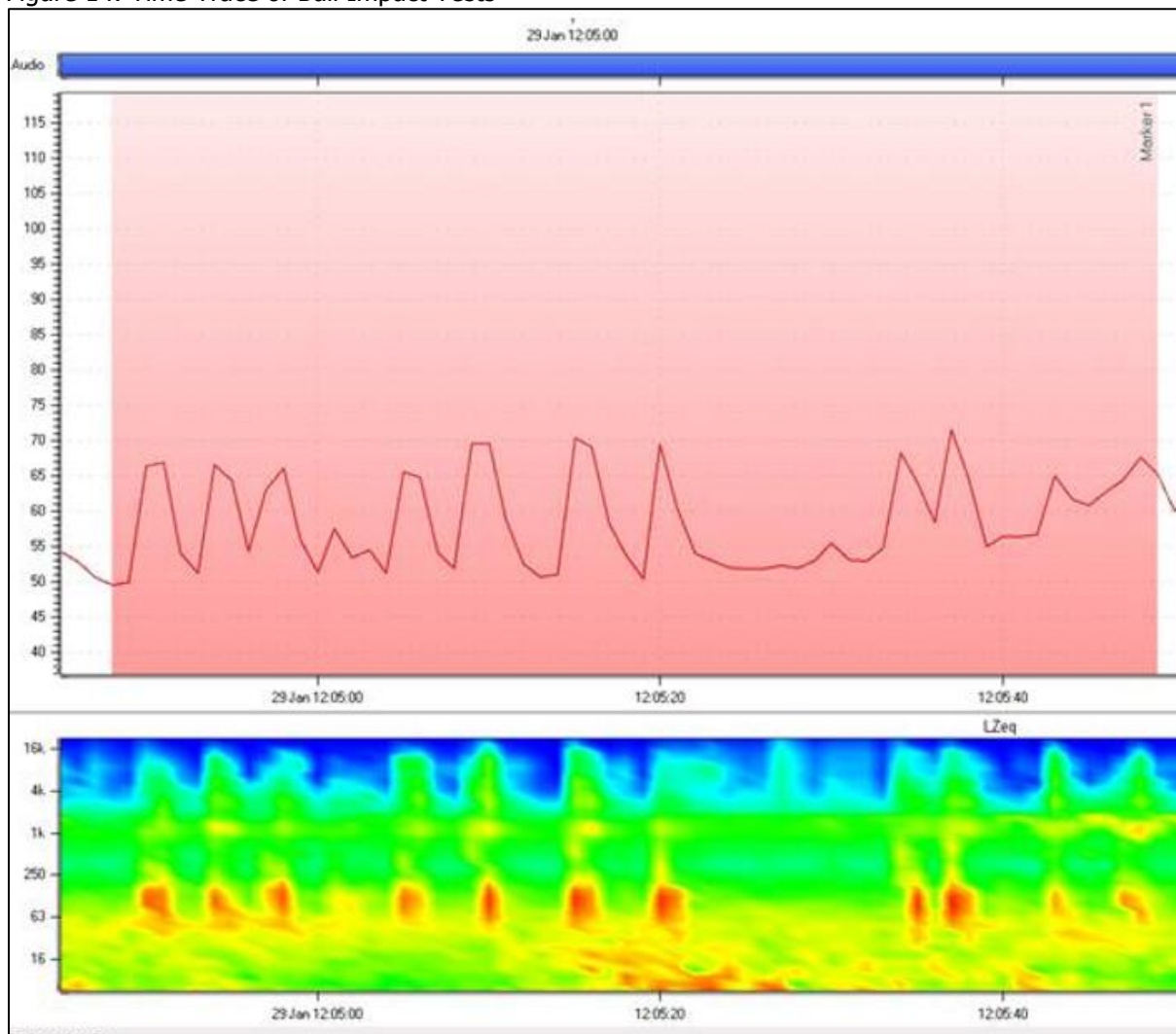
Figure 14: Time Trace of Ball Impact Tests
