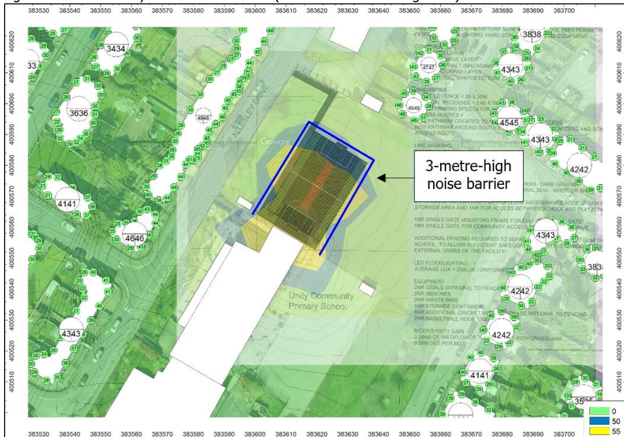
Figure 9: Predicted PlayZone Noise Emission (1.5 metres above the ground)
