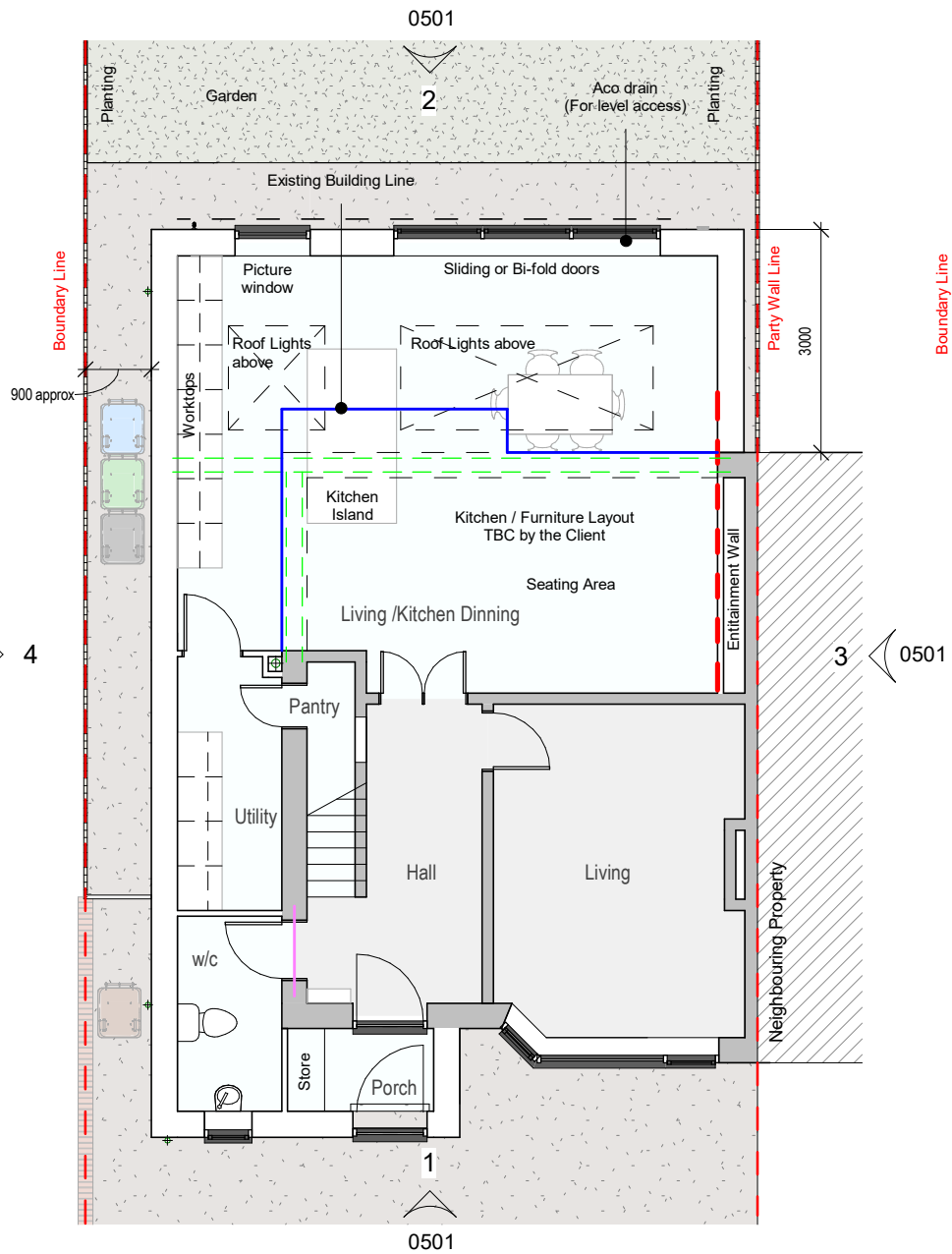
1 | Level 0_Proposed 1 : 100
