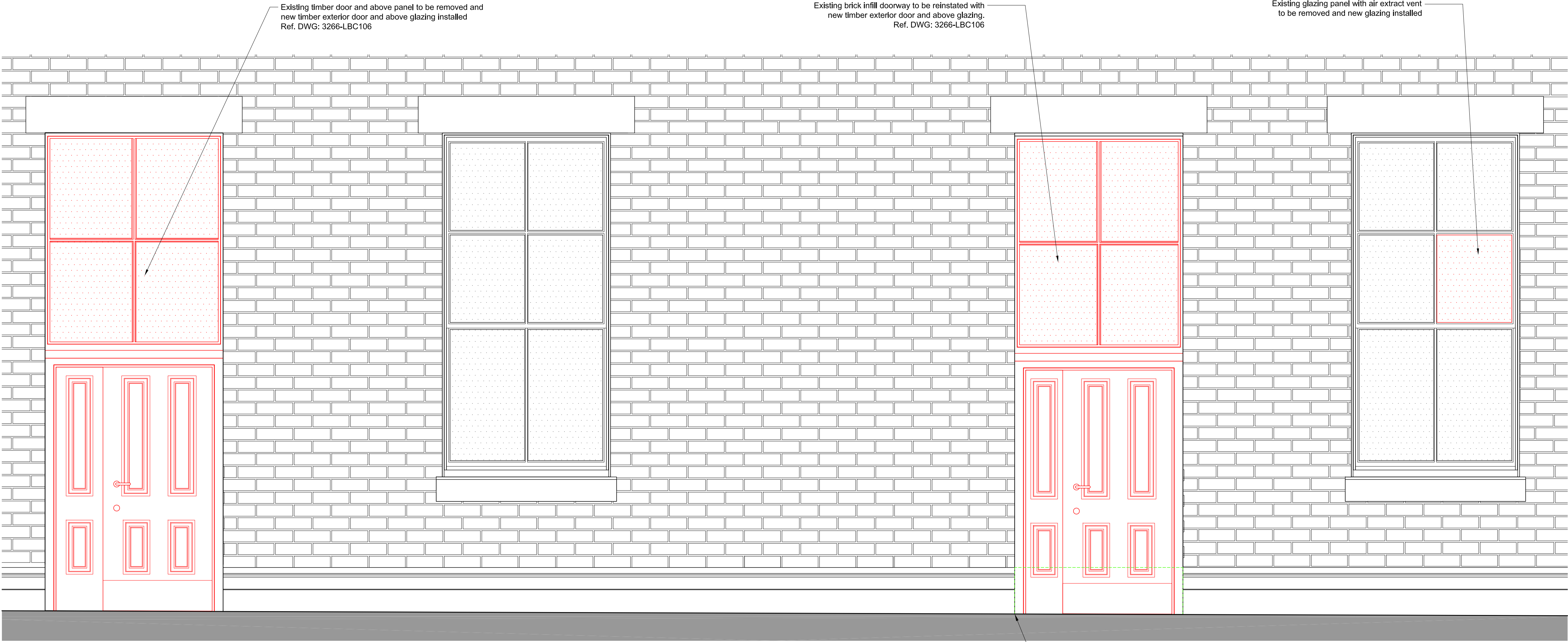
01 PROPOSED PLATFORM 3A BUILDING ELEVATION Scale 1:20 @ A1
