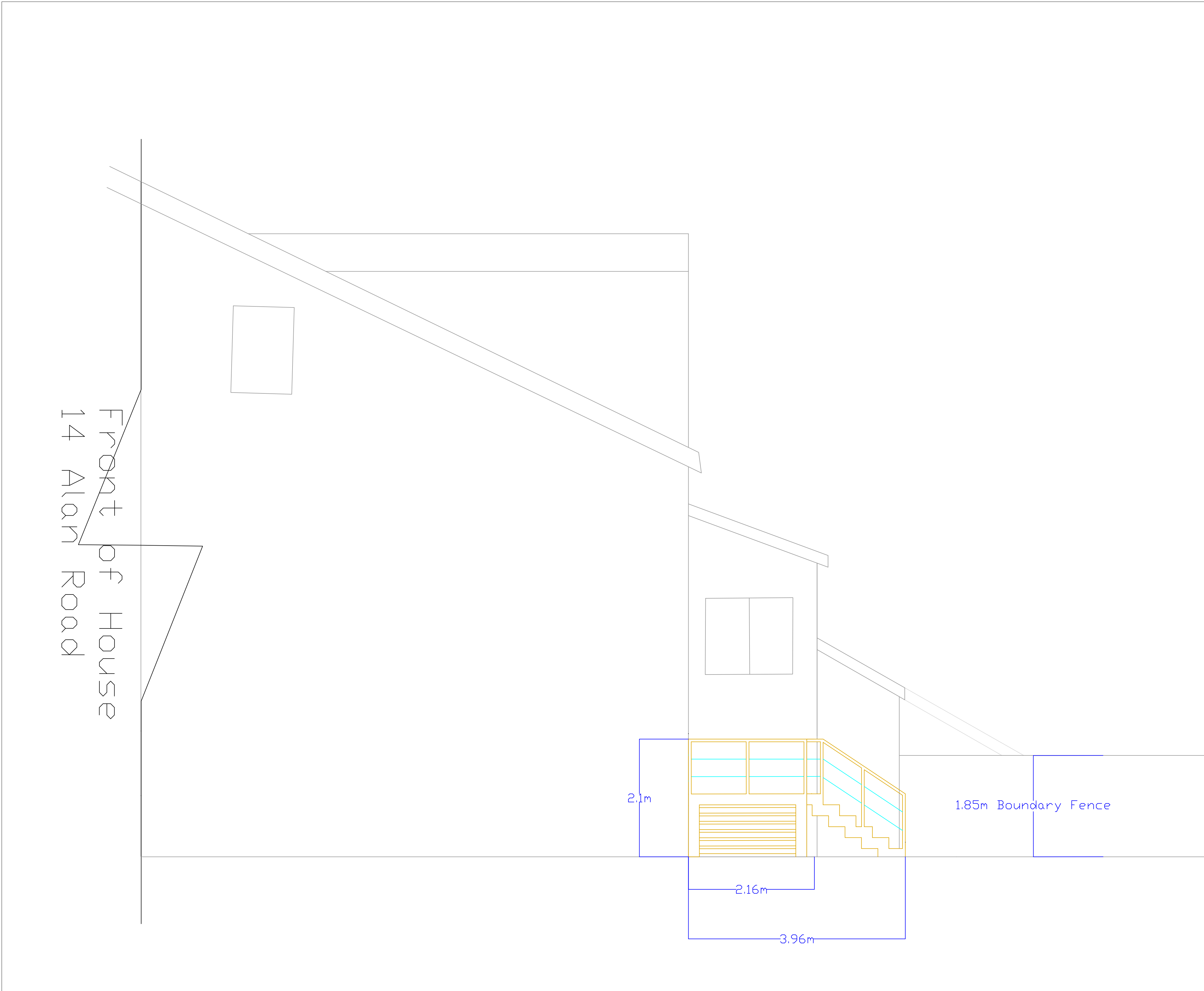
Proposed Side Elevation - From Plot 12 looking to plot 14 but you would have to remove the fence to see this view Scale 1:50@A0
