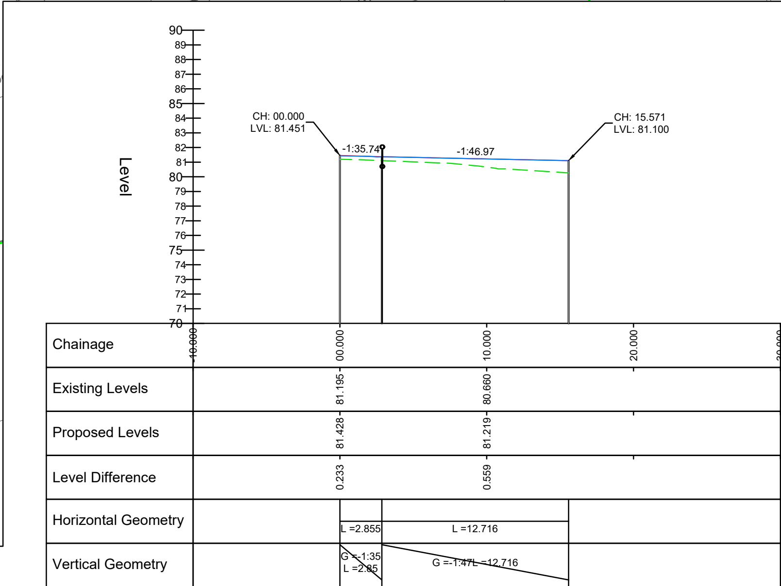
ROAD 2 LONGSECTION SCALE 1:250
