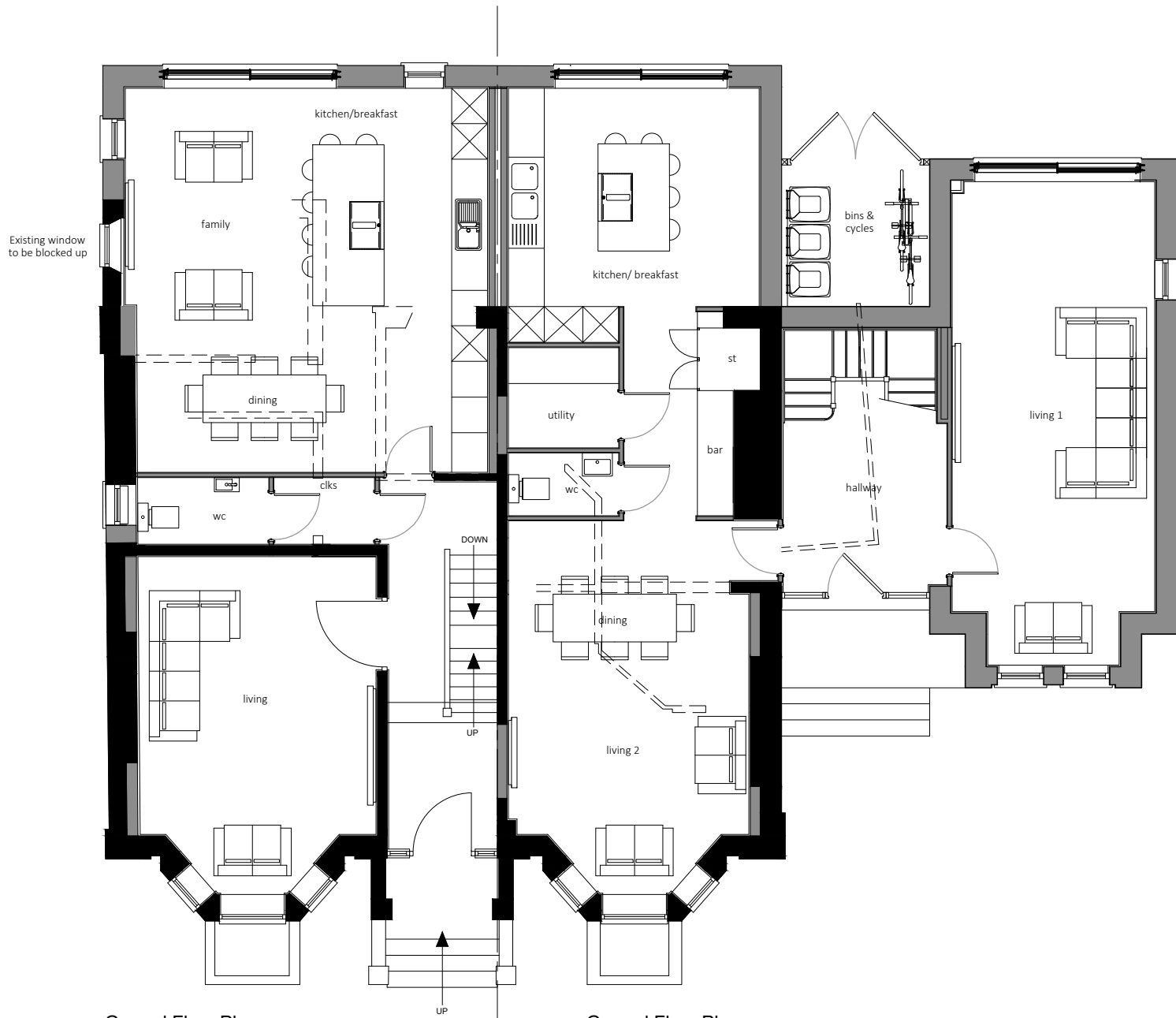
Ground Floor Plan Type D
