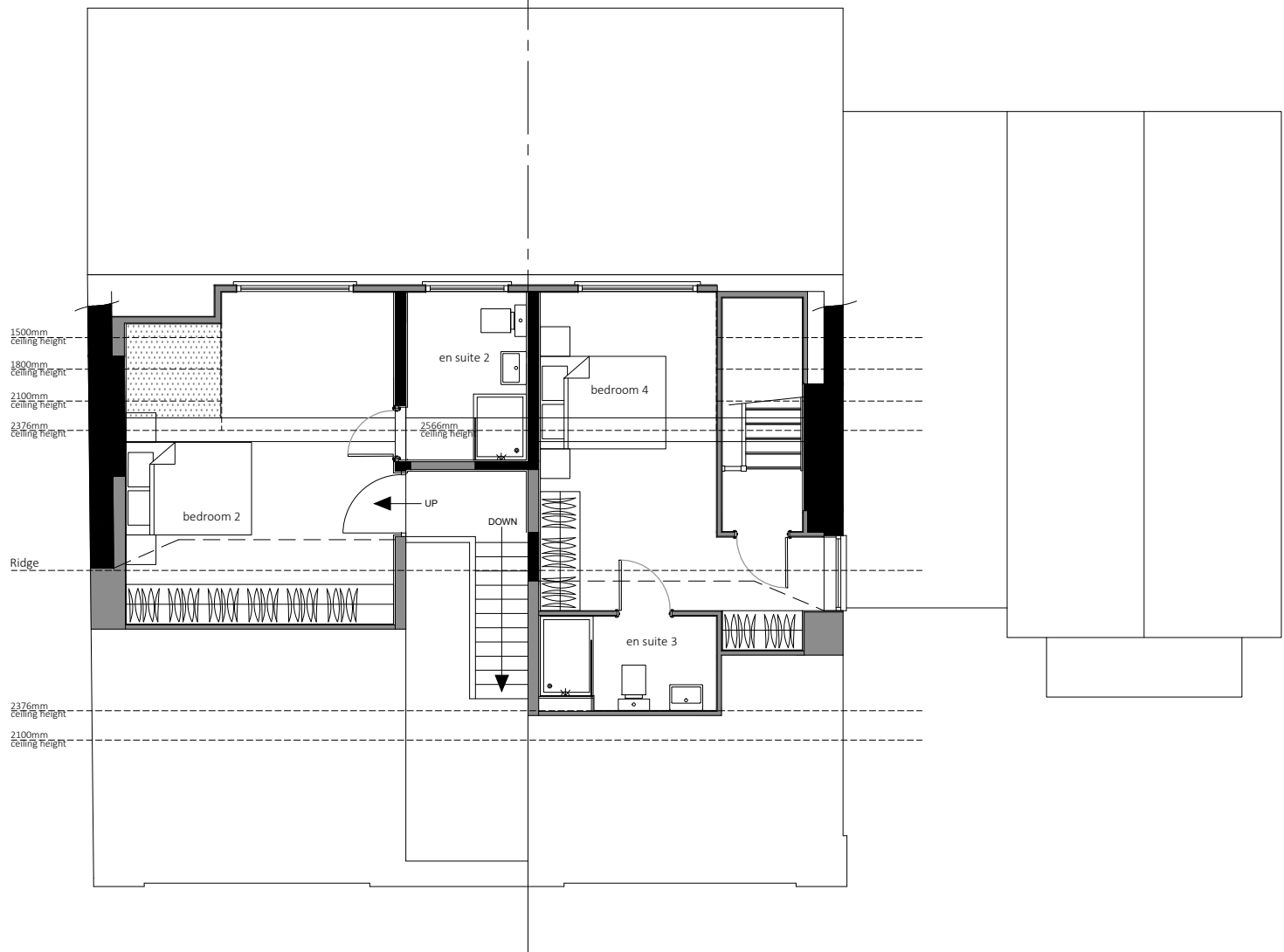
Second Floor Plan Type D
