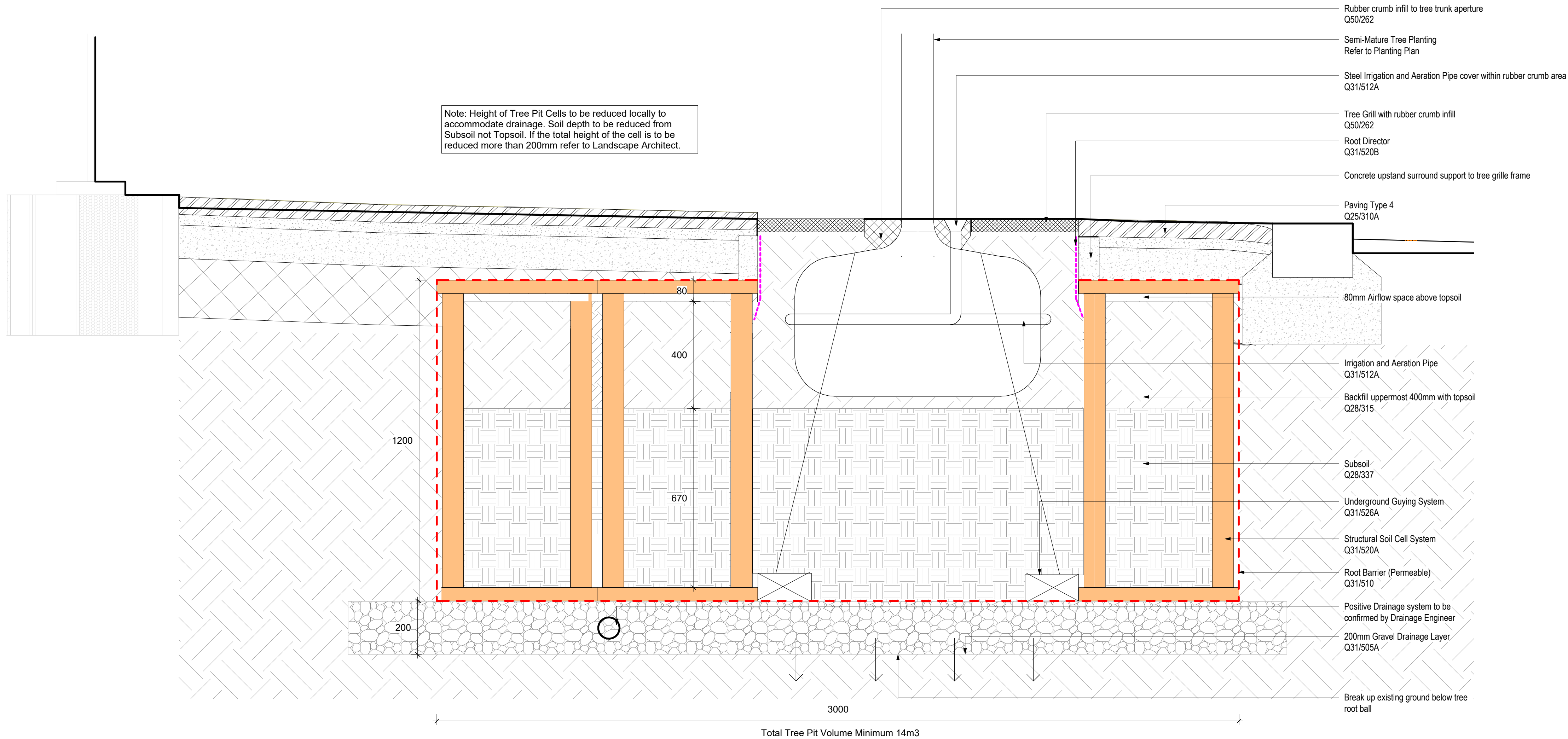
2 000411 Tree Pit Sketch Section 1:10 @
