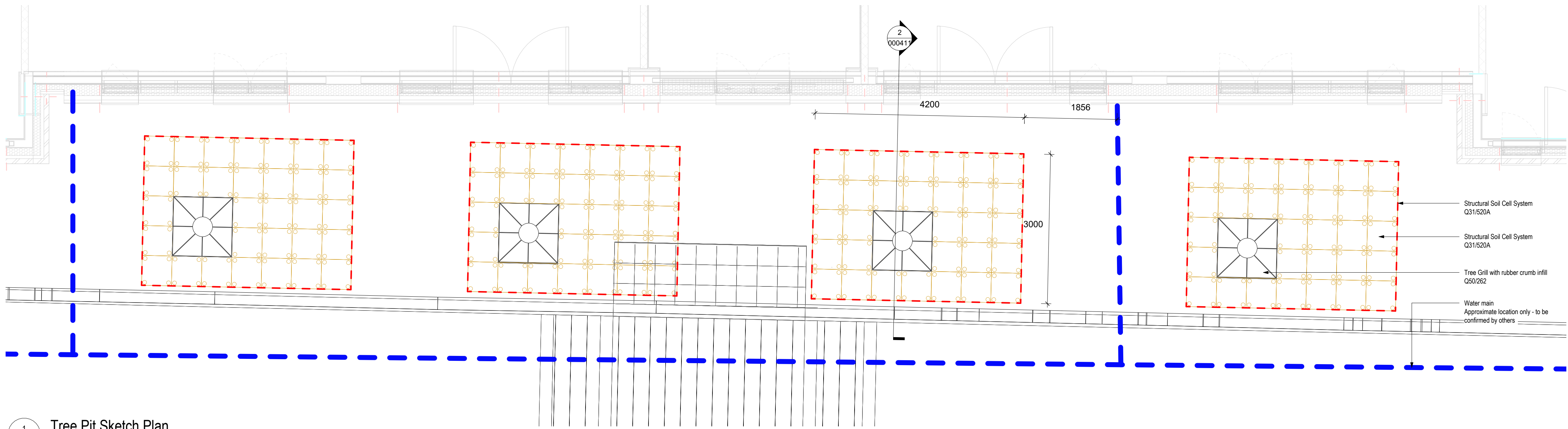
1 000411 Tree Pit Sketch Plan 1:50 @
