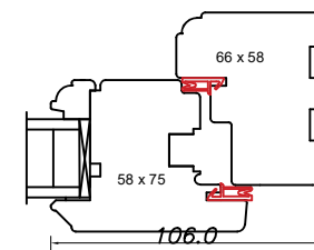
HORIZONTAL SECTION OF WINDOW
