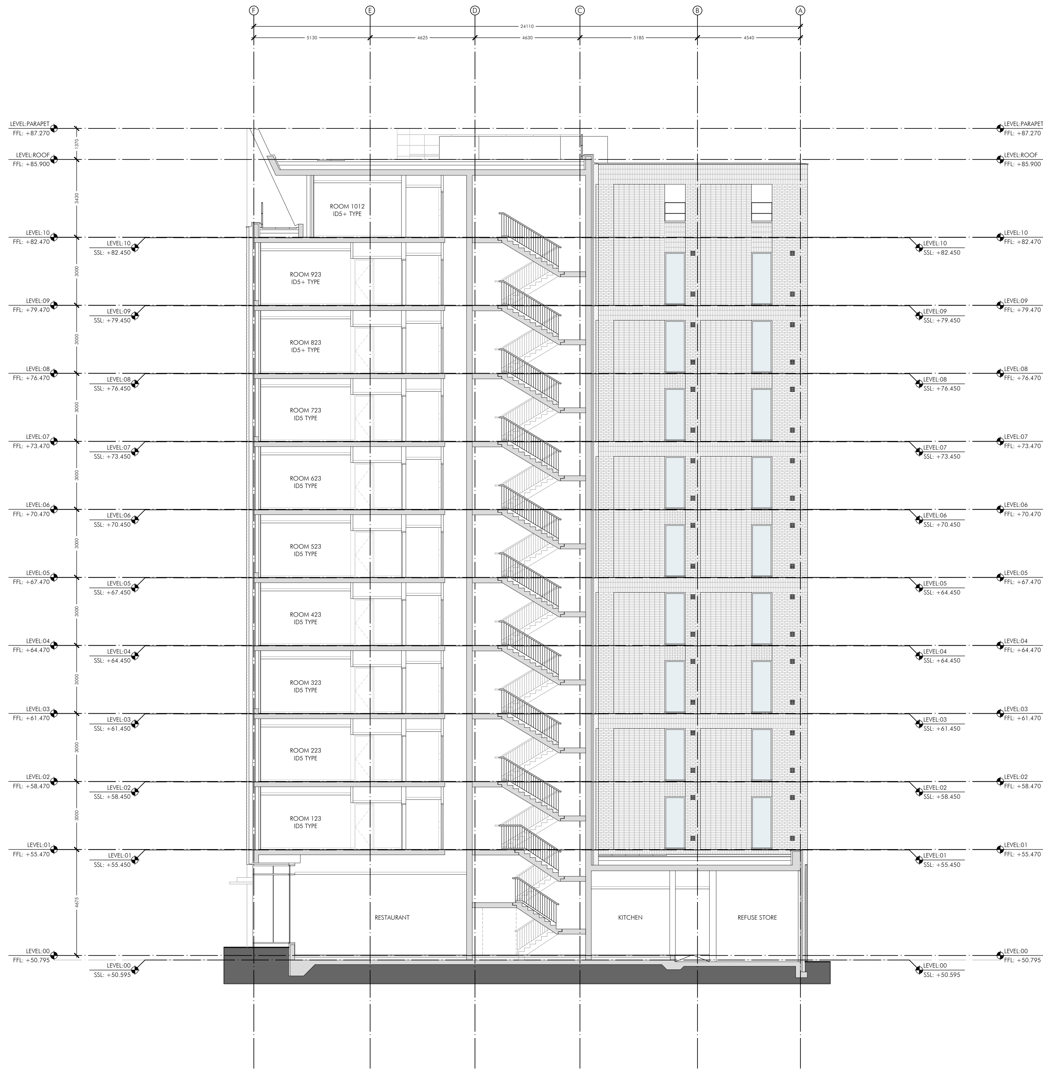
PROPOSED BUILDING SECTION SCALE - 1:100
