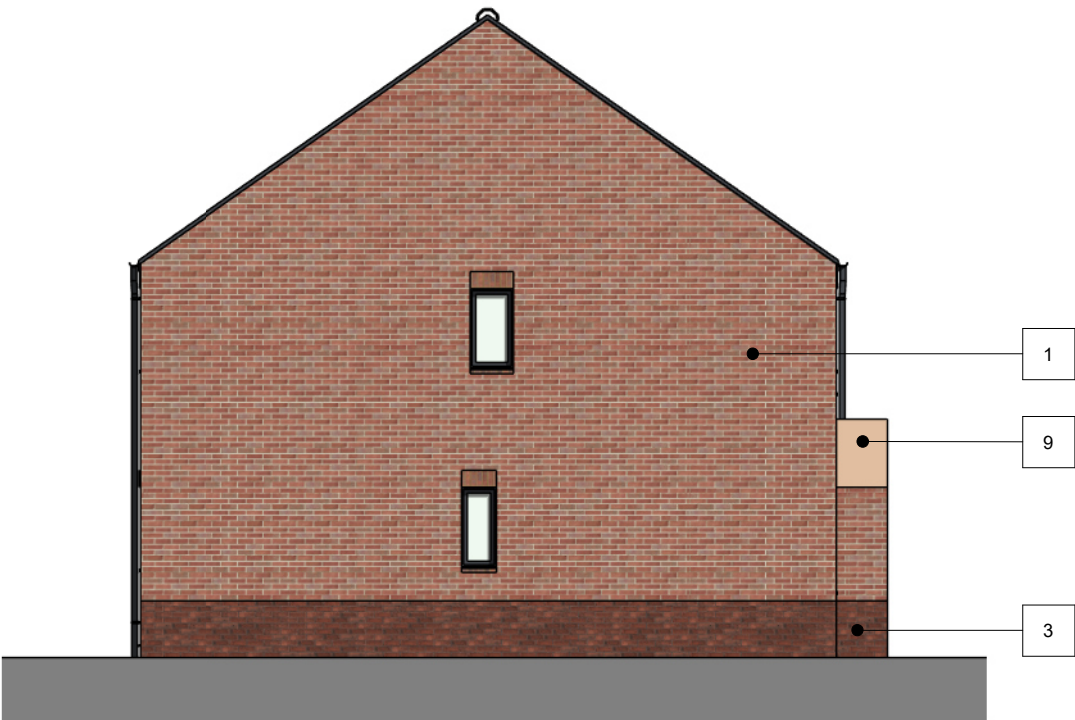
Left Elevation 1 : 100
