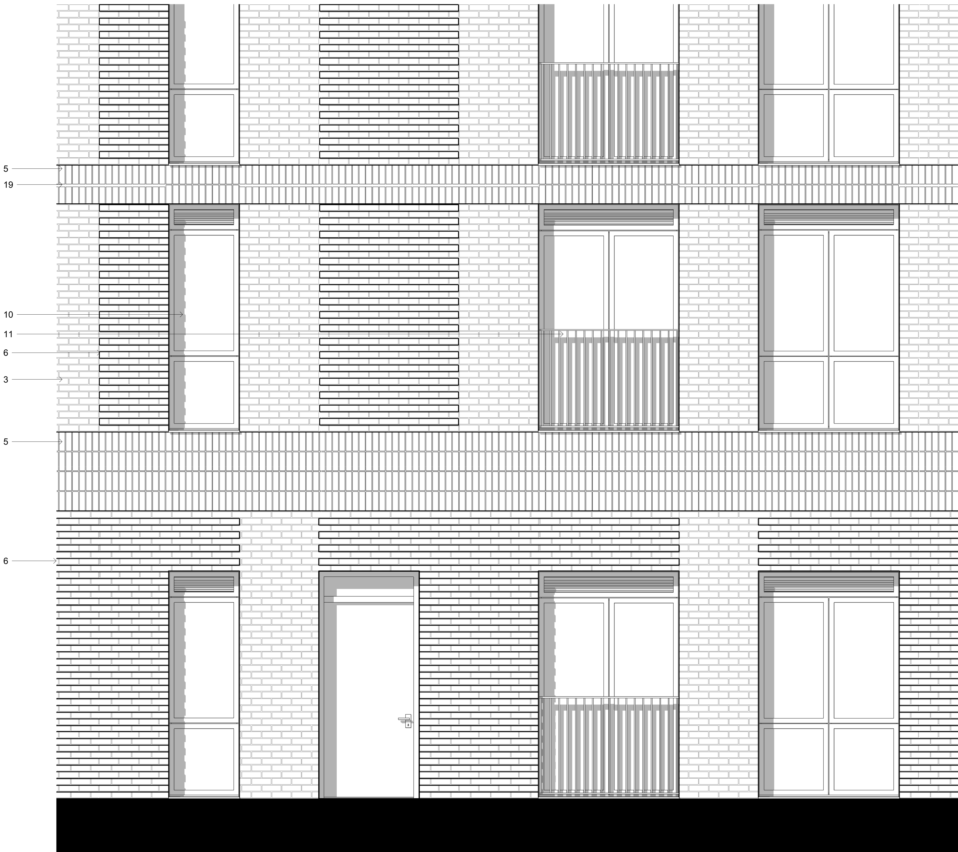
1 Planning Bay Study_East Elevation 1 : 20
