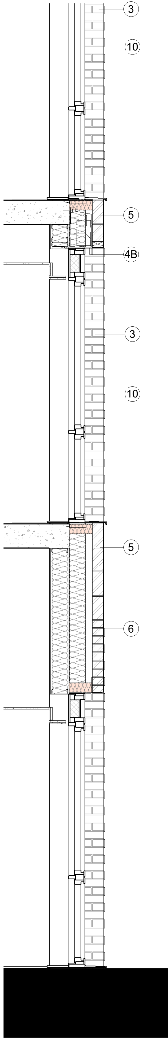
2 Detailed Section 1 : 20
