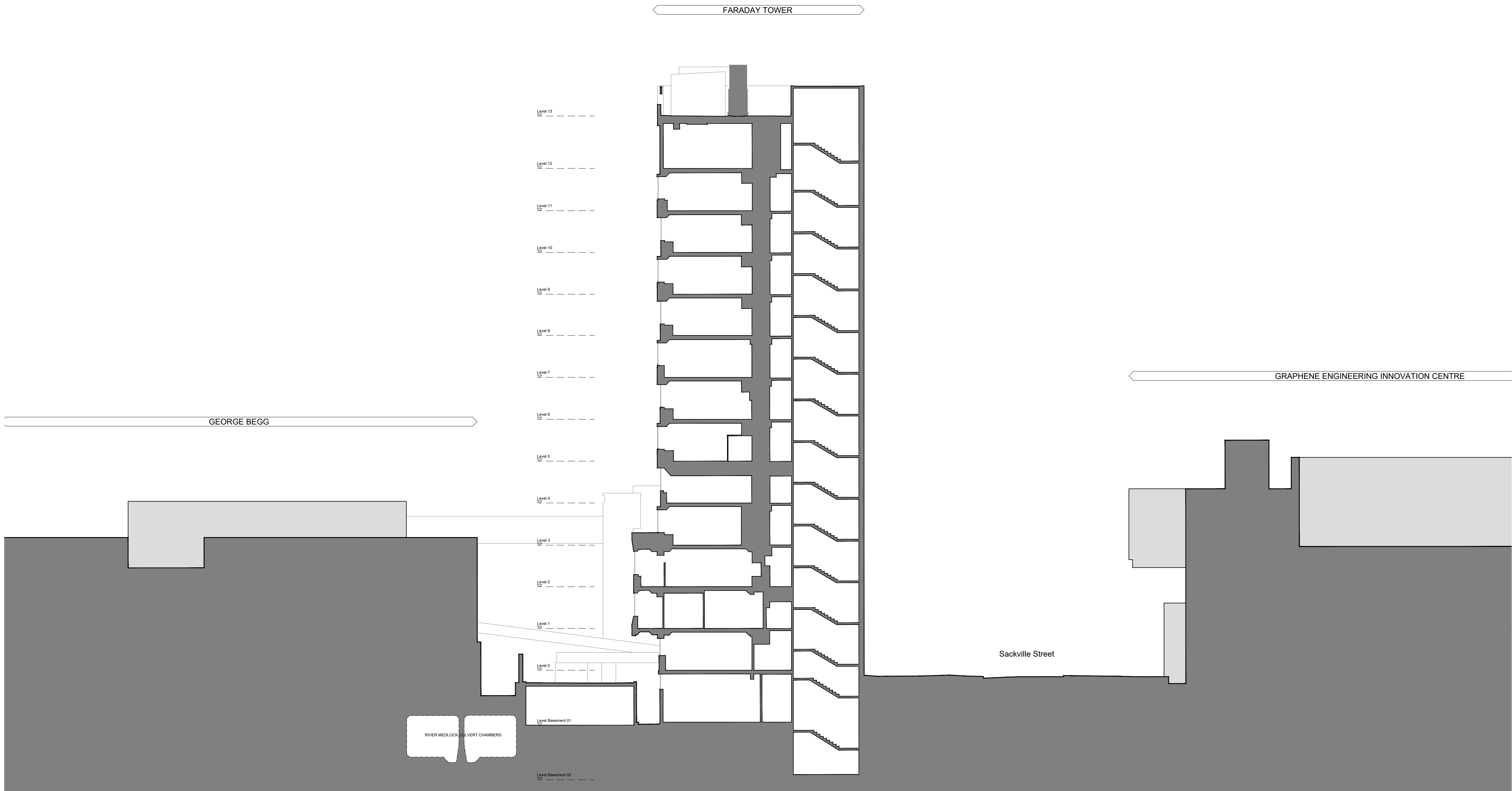
Section B-B
