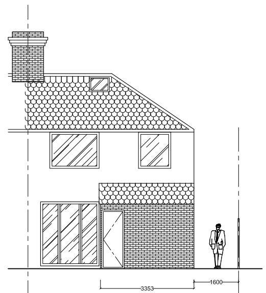
"B - B" Backyard Perspective
