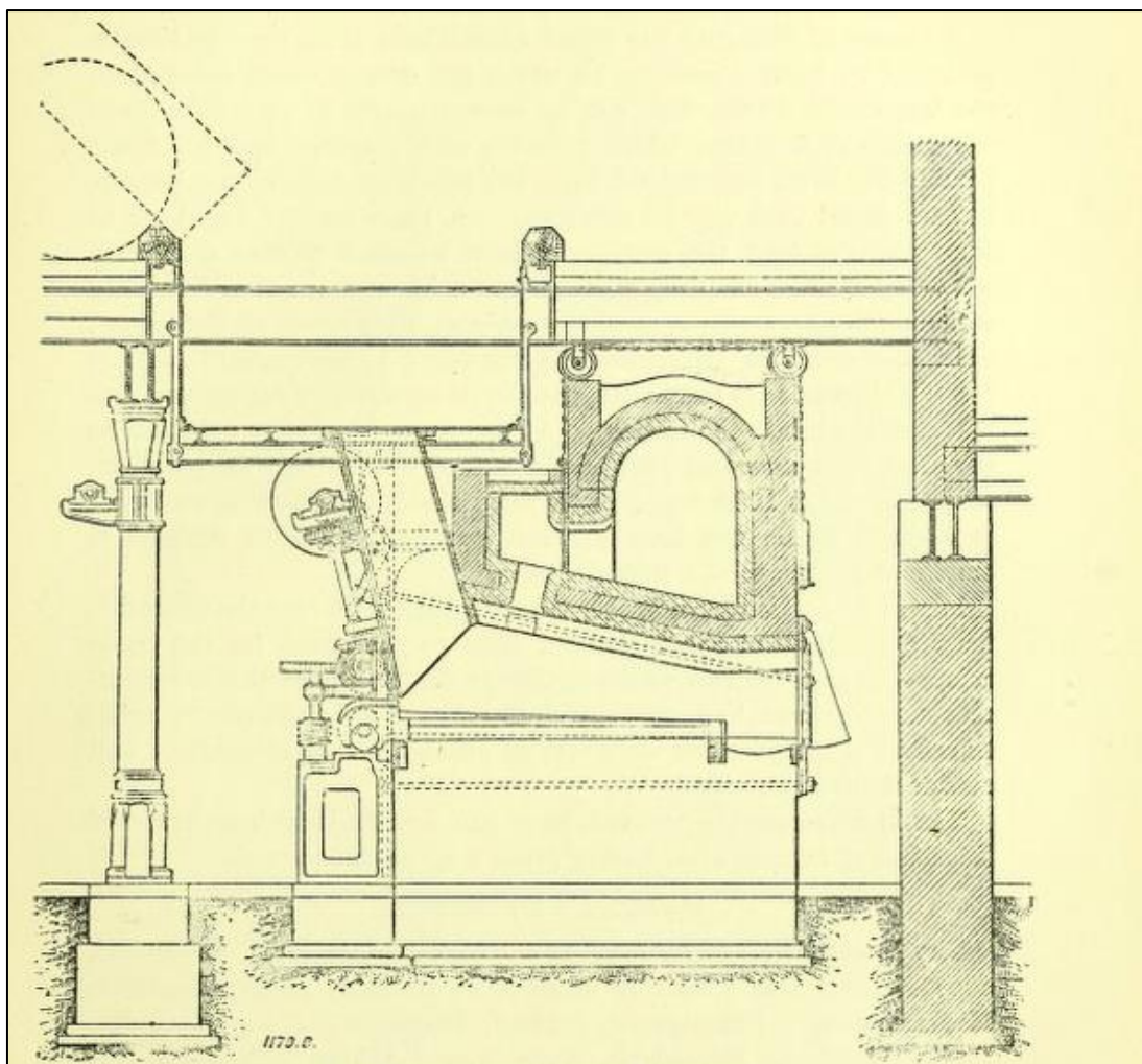
Plate 31: Extract from Maxwell, 'The Removal and Disposal of Town Refuse', showing a cross-section of Whiley's destructor
