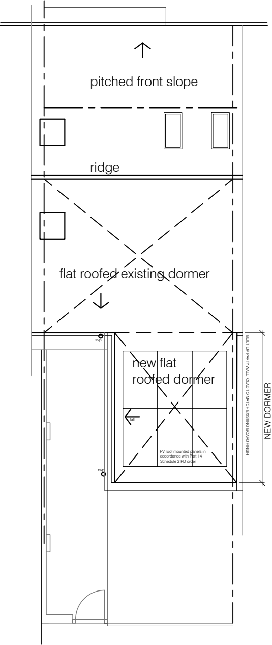
ROOF PLAN
