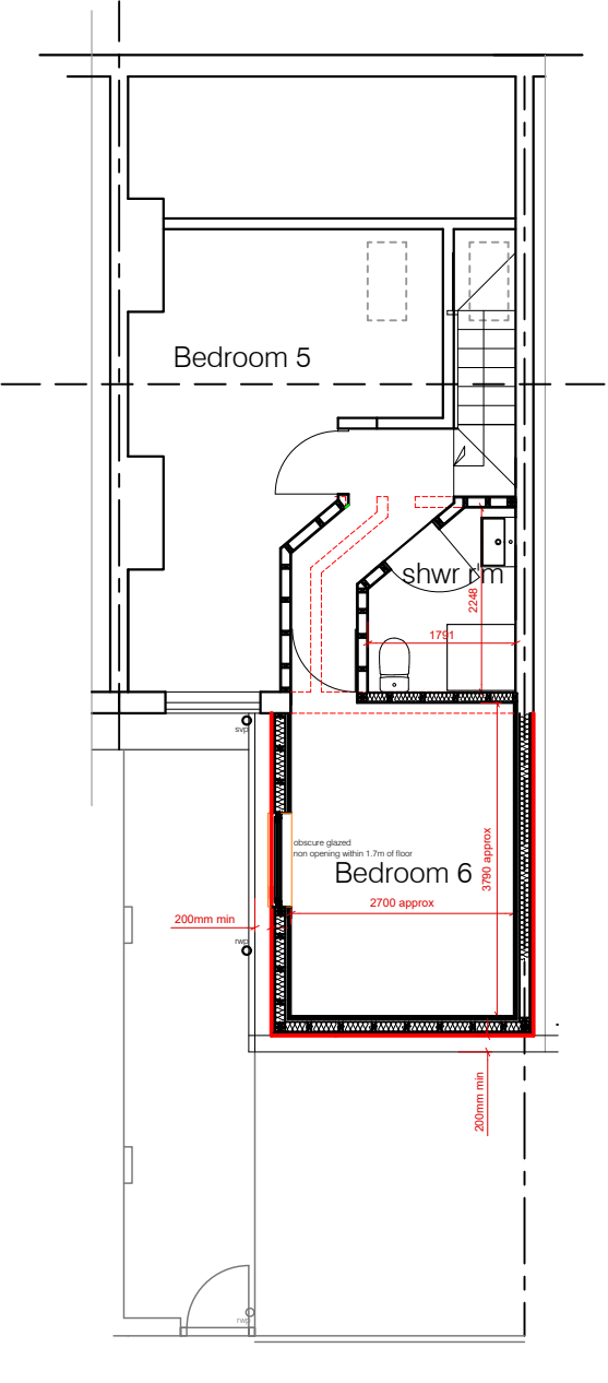
LOFT FLOOR PLAN
