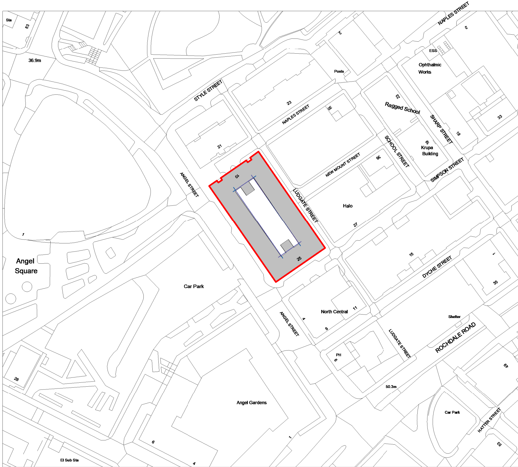
2 Site Location Plan 1 : 1250
