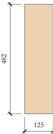
TcW_04 Elevation Left 1 : 10
