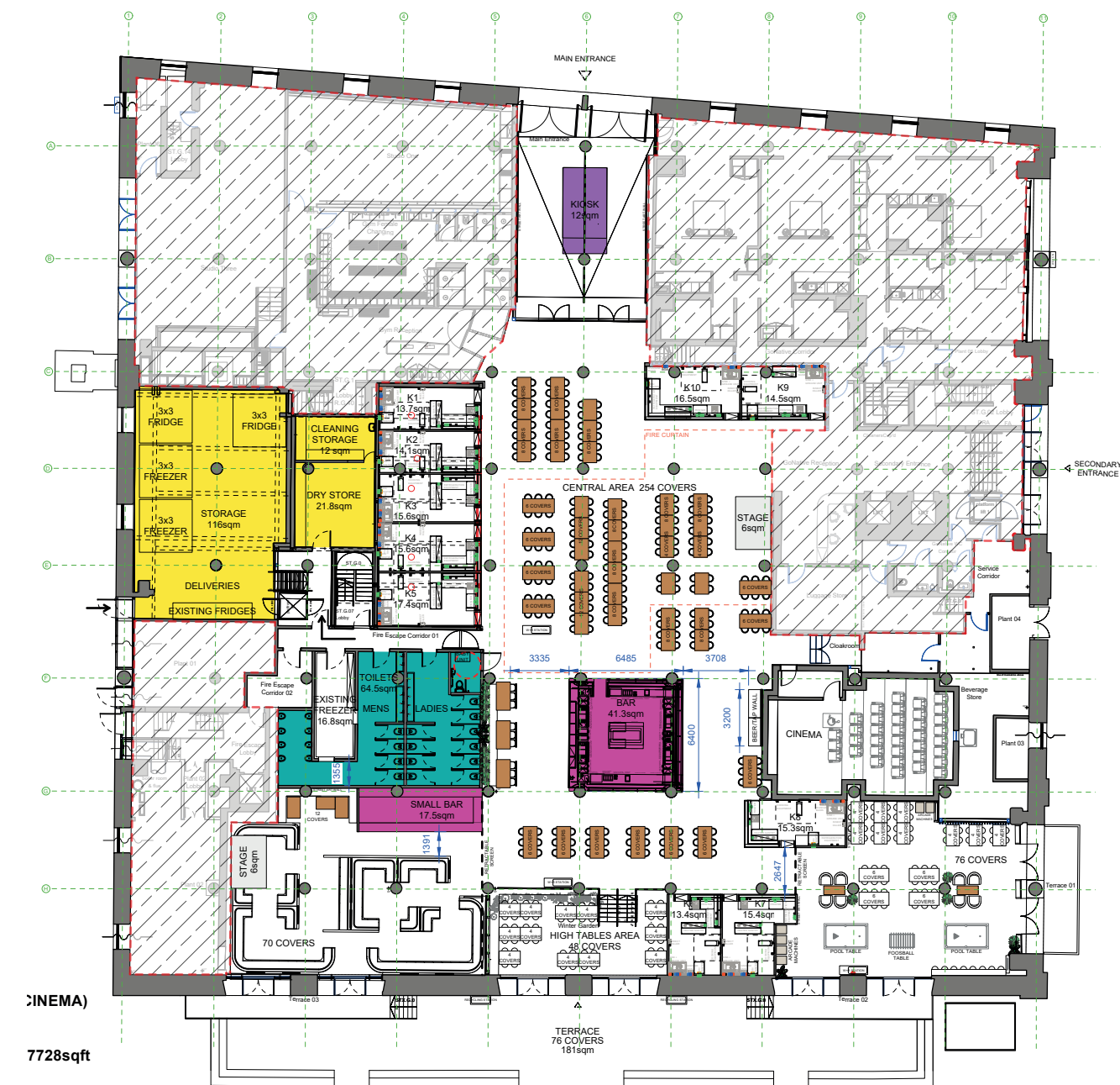
Updated proposed layout
