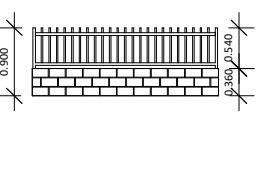
02 Front facing brick wall with mounted metal railing
