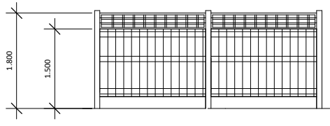
01 Fencing to enclose Private Garden 1500mm high close boarded timber fence with 300mm trellis with concrete post and gravel board to all private rear gardens to a total height of 1800mm
