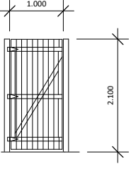
04 Pedestrian Gate to Private Garden 1000 x 2100mm high close- boarded timber gate
