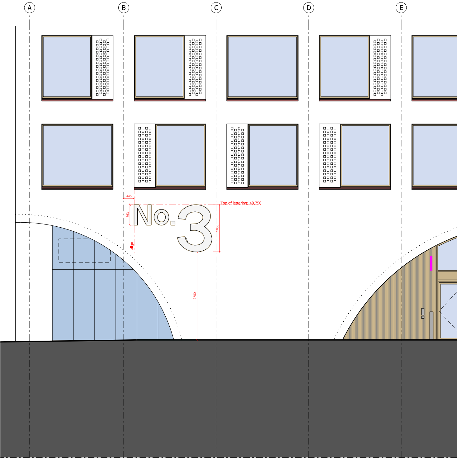
WEST ELEVATION (extract)
