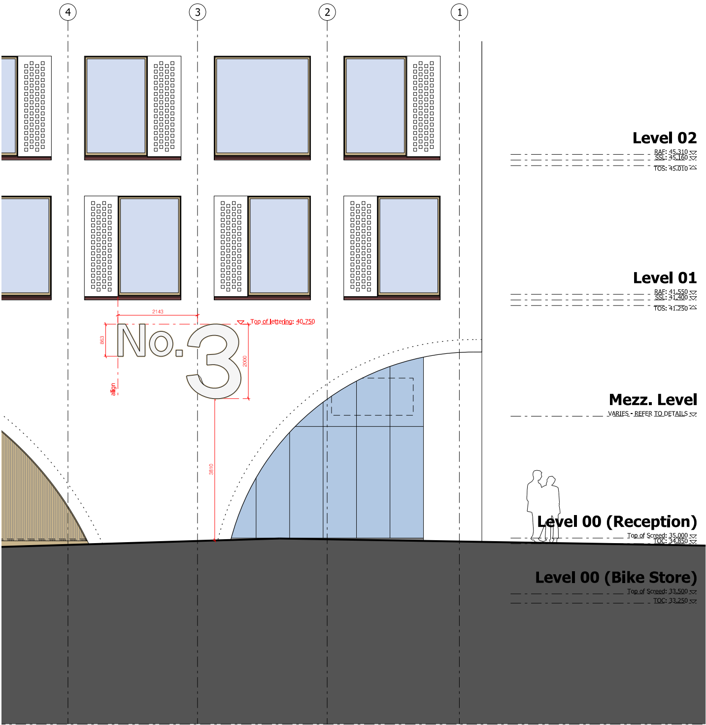
SOUTH ELEVATION (extract)
